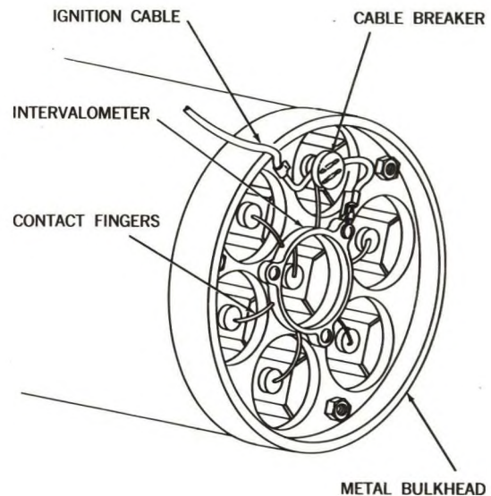
Figure 7-3. Ignition System.
