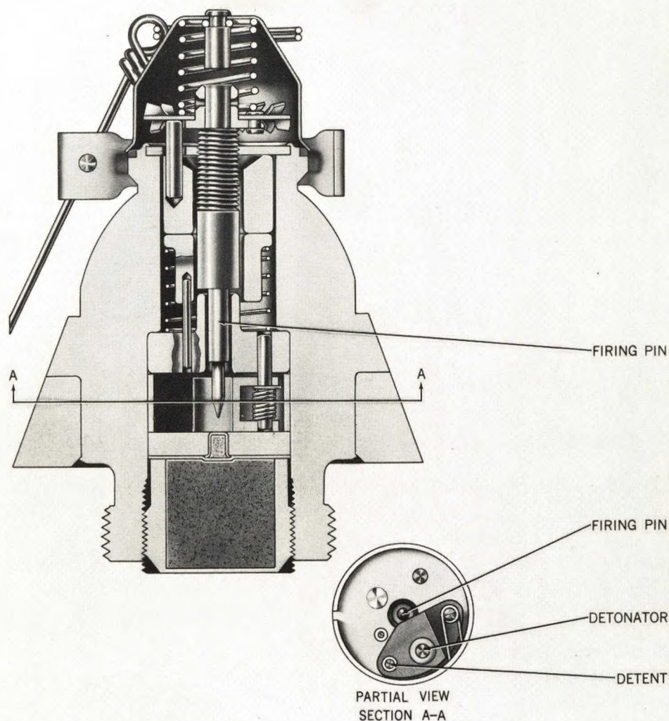
Figure 4-2. Nose Fuze Mk 149 Mod 1, Cross Section, Unarmed Position.
