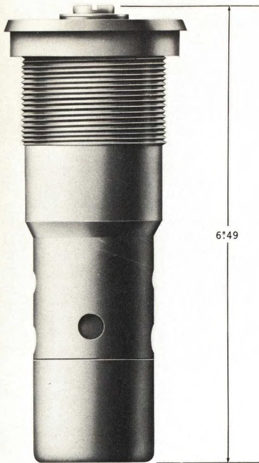
Figure 4-15. Base Fuze Mk 166 Mod 2, External View.
