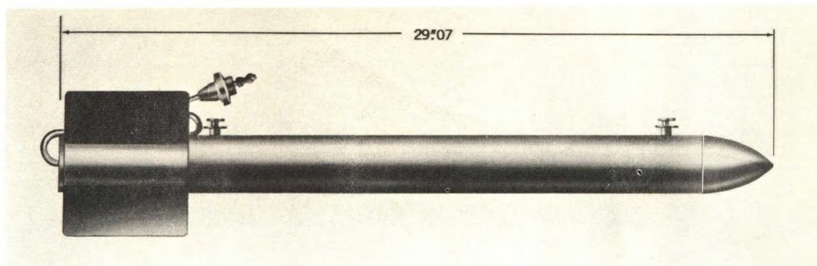
Figure 5-2. 2.25-Inch Rocket Mk 6 Mod 0 (SCAR), External View.
