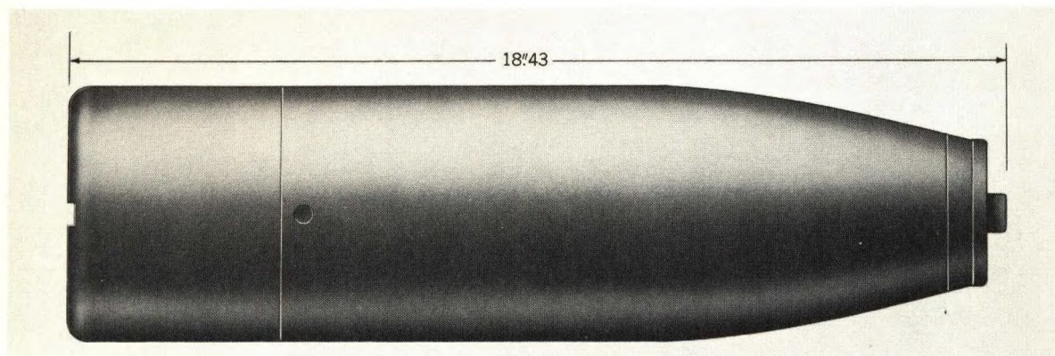
Figure 2-9. 5.0-Inch Rocket Warhead Mk 6 Mod 4 (VT), External View.
