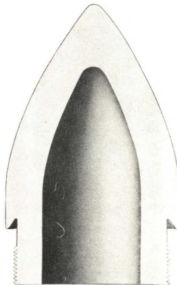
Figure 2-2. 2.25-Inch Rocket Head Mk 3 Mod 3 (PRAC, SC), Cross Section.
