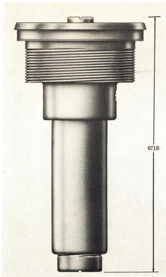
Figure 4-12. Base Fuze Mk 164 Mod 0, External View.
