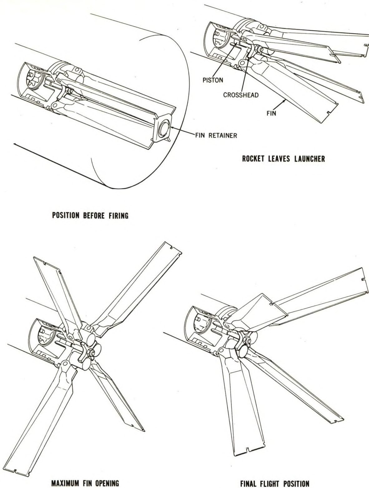
Figure 1-21. Phases of Fin Assembly Functioning, 2.75-Inch Folding-Fin Aircraft Rocket.
