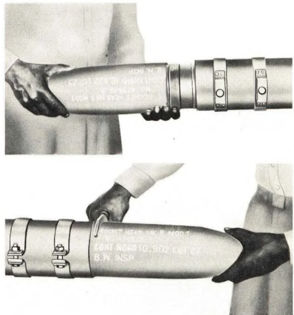
Figure 1-26. Threading Head into Motor of 5-Inch HVAR Rocket; Starting the Threading by Hand (top), and Seating the Head with Spanner Wrench (bottom).
