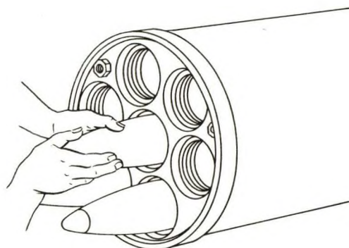
Figure 7-8. Rocket Head Installation.
