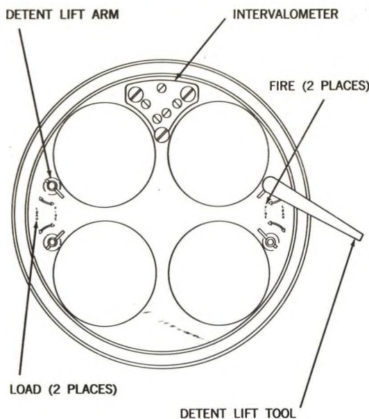
Figure 7-14. Launcher Forward Bulkhead.
