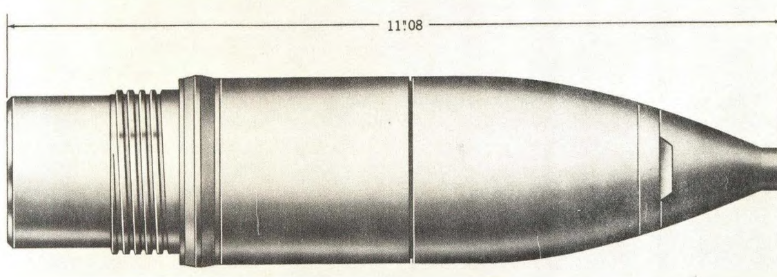
Figure 2-5. 2.75-Inch Rocket Warhead Mk 5 Mod 0 (HEAT), External View.
