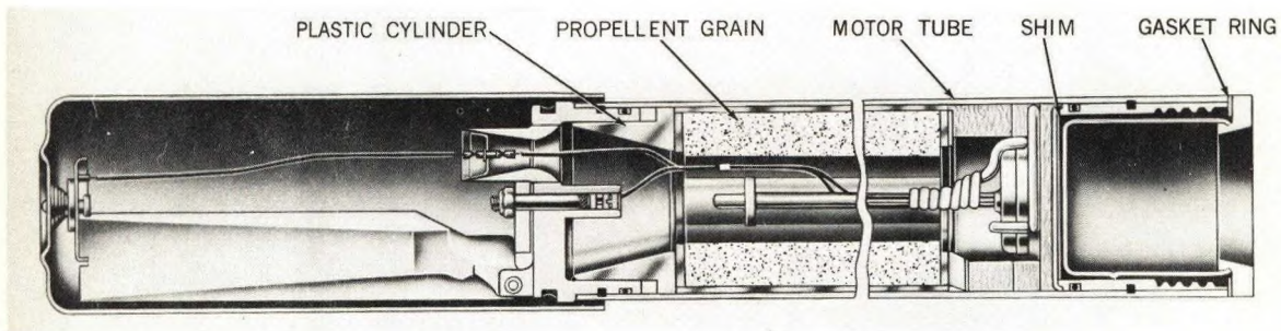
Figure 3-15. 2.75-Inch Rocket Motor Mk 3 Mod 3, Sectional View.
