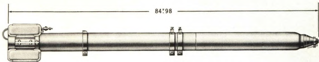
Figure 5-15. 5.0-Inch Rocket Mk 36 Mod 0 (SMOKE-PWP, HVAR), External View.
