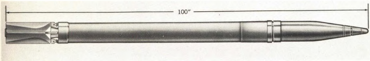
Figure 5-17. 5.0-Inch Folding-Fin Aircraft Rocket (ZUNI) Mk 40 Mod 1, Ready for Firing.
