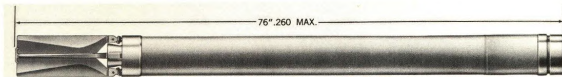
Figure 3-20. 5.0-Inch Rocket Motor Mk 16 Mod 1, External View.
