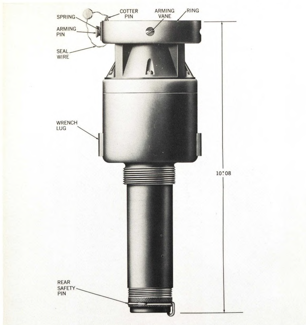
Figure 4-3. Nose (VT) Fuze Mk 172 Mod 2, External View.
