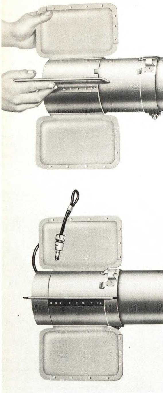
Figure 1-25. Installing Fin Assembly on 5-Inch HVAR Motor; Placing Fin Assembly on Motor Tube (top), and Secured Position of Fin Assembly (bottom).
