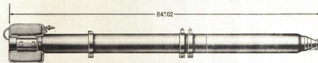
Figure 5-12. 5.0-Inch Rocket Mk 32 Mod 1 (HEAT, HVAR), External View.
