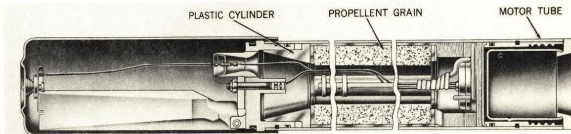
Figure 3-13. 2.75-Inch Rocket Motor Mk 3 Mod 4, Sectional View, with Fin Retainer in Place.
