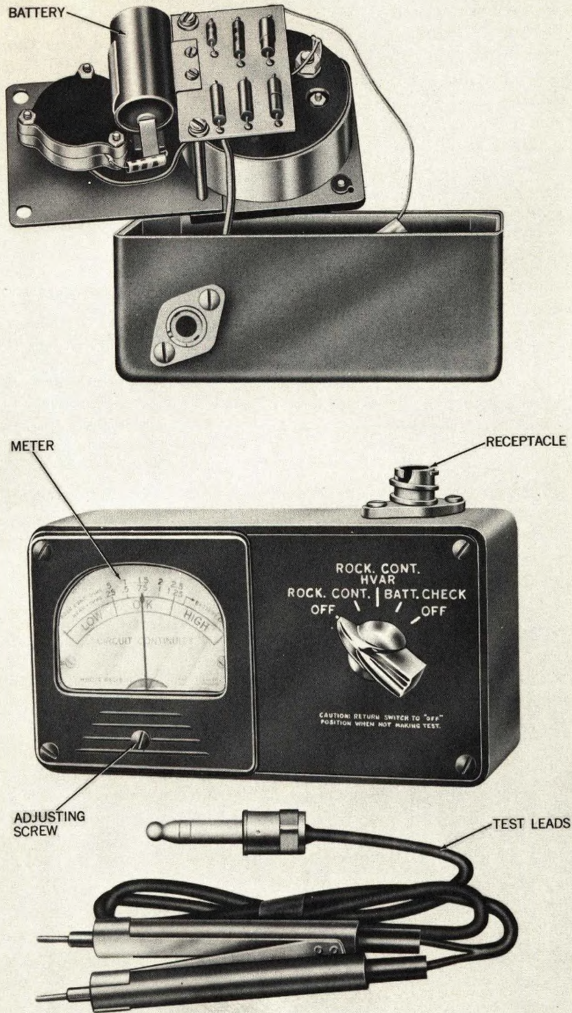
Figure 8-2. Circuit Continuity Tester Model 680B, Disassembled, External View, and Test Leads.
