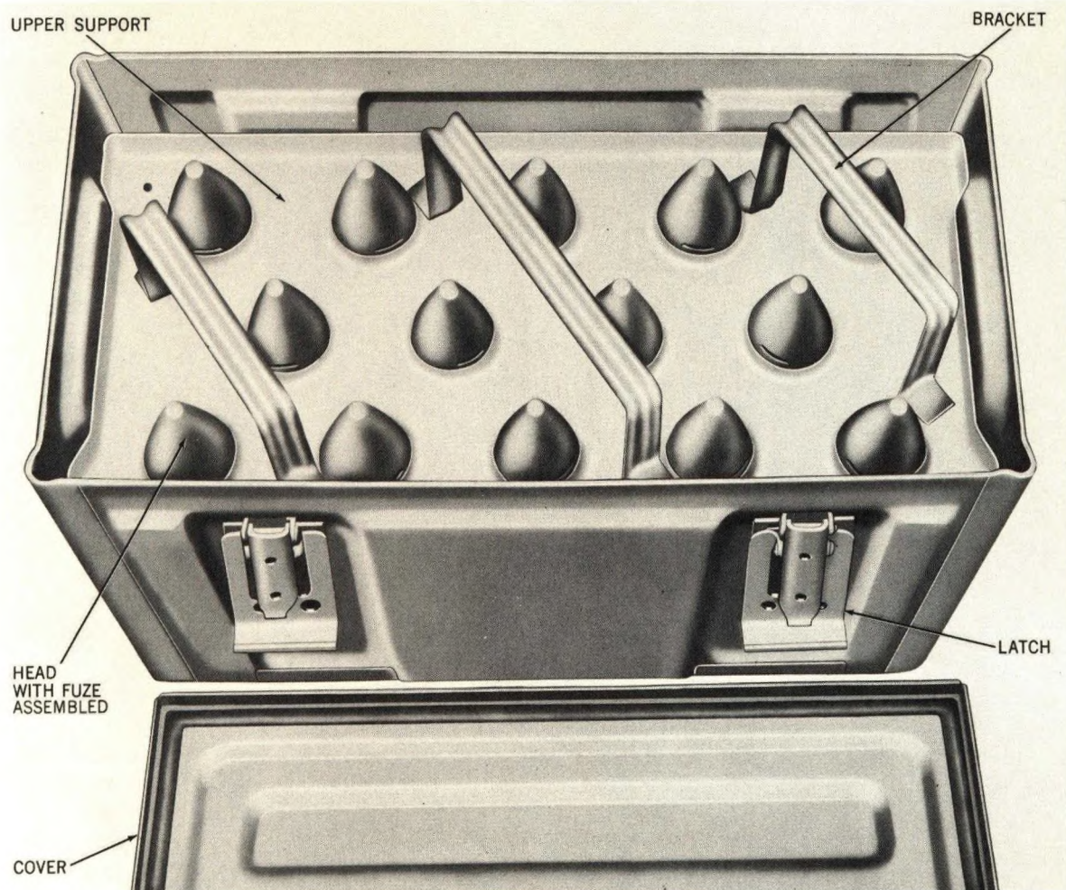
Figure 1-19. Typical Head Container for 2.75-Inch Rockets, Cover Removed.
