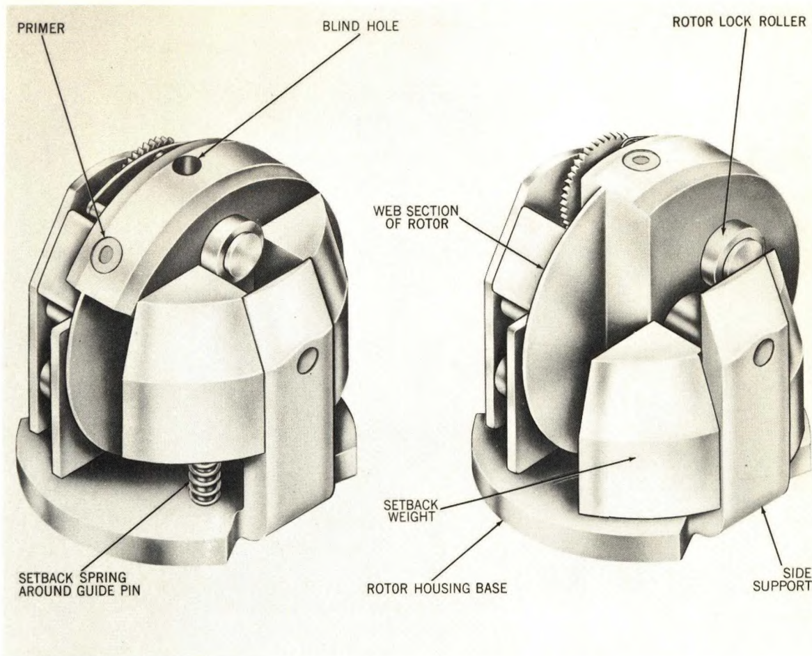
Figure 1-9. Rotor Arming Mechanism Removed from Fuze, Unarmed and Armed Positions, View from Right-hand Side.
