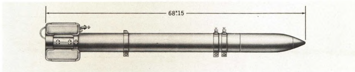
Figure 5-16. 5.0-Inch Rocket Mk 39 Mod 0 (PRAC, HVAR), External View.
