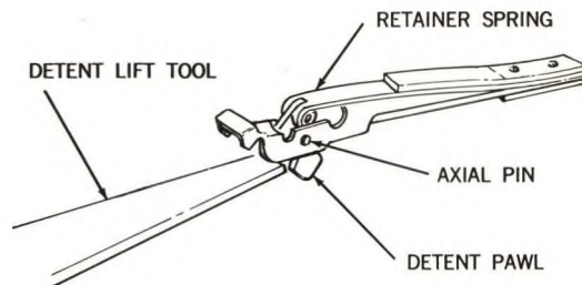
Figure 7-16. Detent Relatching.
