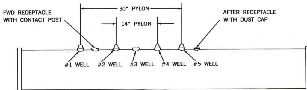
Figure 7-15. Hanger and Receptacle Arrangement.
