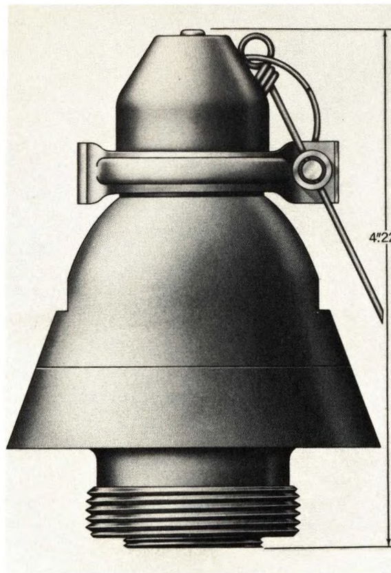
Figure 4-1. Nose Fuze Mk 149 Mod 1, External View.
