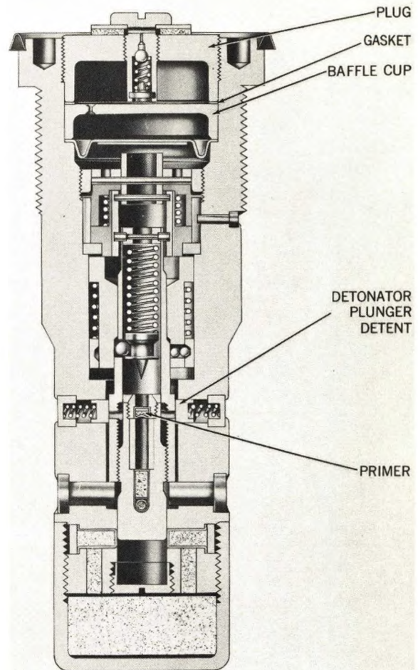
Figure 4-16. Base Fuze Mk 166 Mod 2, Cross Section, Unarmed Position.
