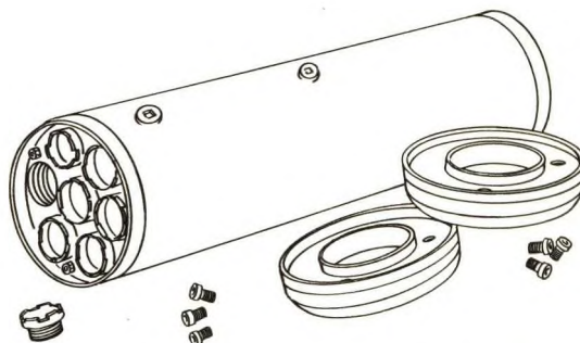
Figure 7-5. Motor Lock Plug Removal.
