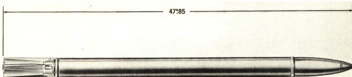
Figure 5-7. 2.75-Inch Rocket Mk 6 Mod 1 (HE-FFAR), Ready for Firing.
