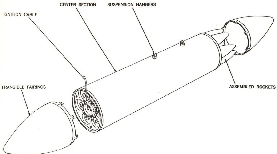
Figure 7-2. Rocket Launcher, Flight Configuration.
