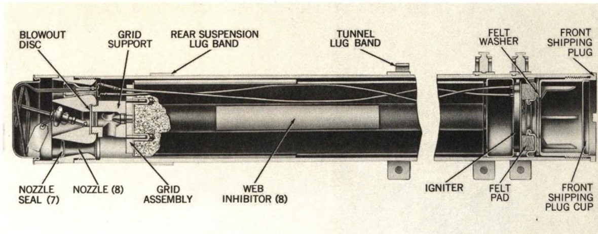
Figure 3-19. 5.0-Inch Rocket Motor Mk 10 Mod 6, Cross Section.
