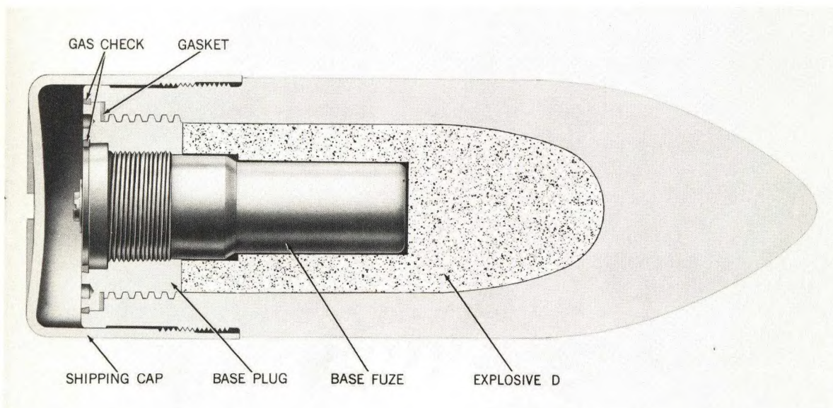
Figure 2-7. 5.0-Inch Rocket Warhead Mk 2 Mod 2 (AP), Cross Section.
