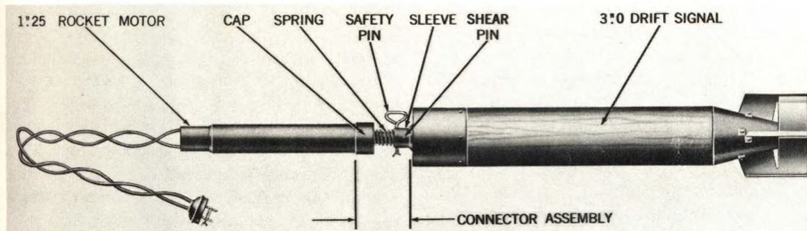
Figure A-2. 3.0-Inch Rocket Mk 16 Mod 1 (Aircraft, Night Drift Signal, RETRO-200 fps).
