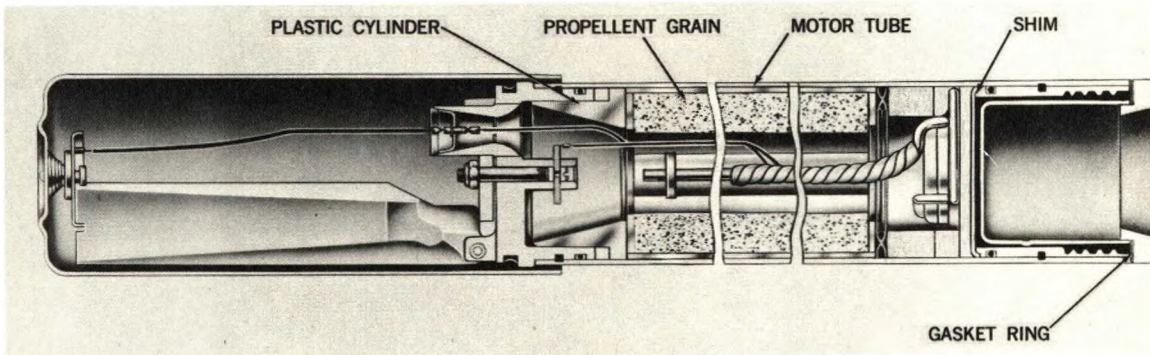
Figure 3-17. 2.75-Inch Rocket Motor Mk 4 Mod 0, Sectional View.
