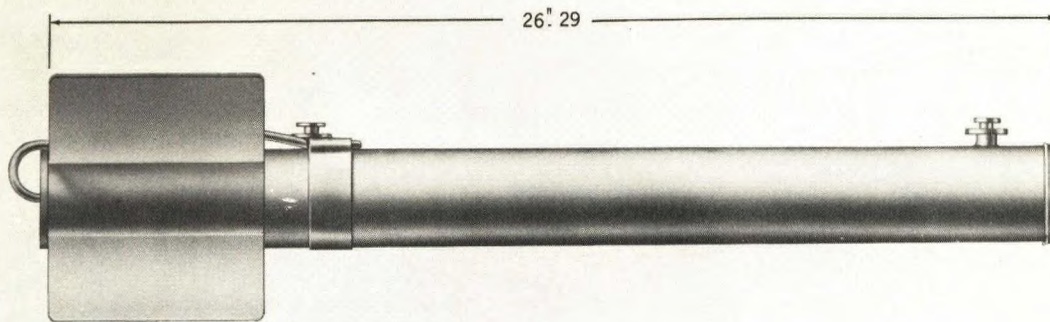
Figure 3-3. 2.25-Inch Rocket Motor Mk 16 Mod 6, External View.
