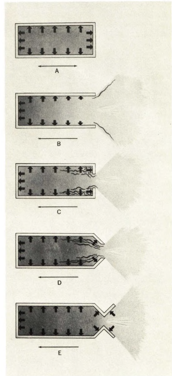
Figure 1-1. Principles of Rocket Propulsion.
