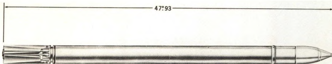
Figure 5-8. 2.75-Inch Rocket Mk 7 Mod 0 (HEAT-FFAR), Ready for Firing.
