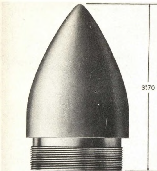
Figure 2-1. 2.25-Inch Rocket Head Mk 3 Mod 3 (PRAC, SC), External View.
