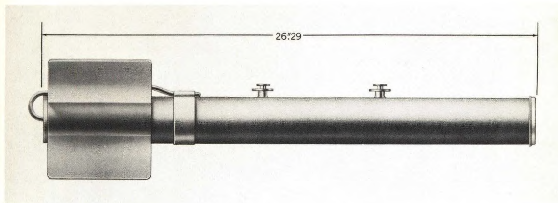
Figure 3-1. 2.25-Inch Rocket Motor Mk 15 Mod 2, External View.
