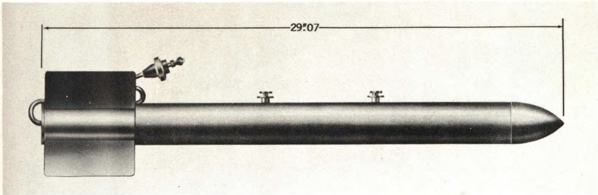
Figure 5-1. 2.25-Inch Rocket Mk 4 Mod 0 (SCAR), External View.
