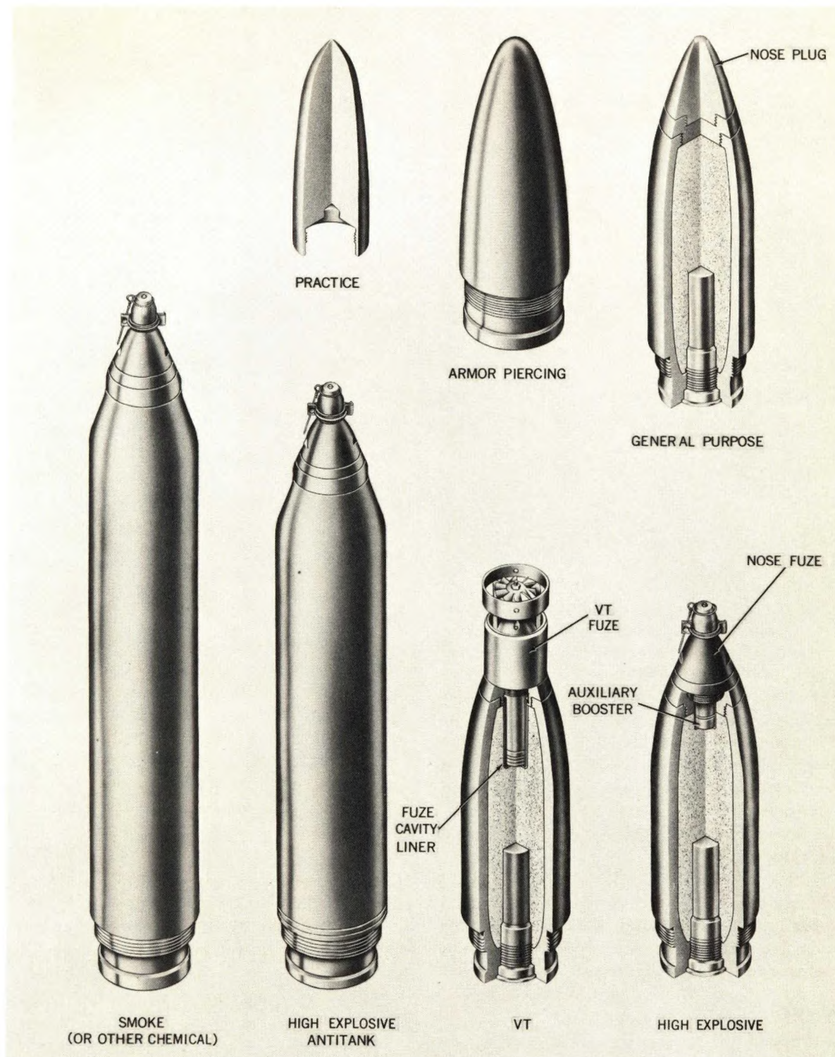
Figure 1-3. Types of Rocket Heads.
