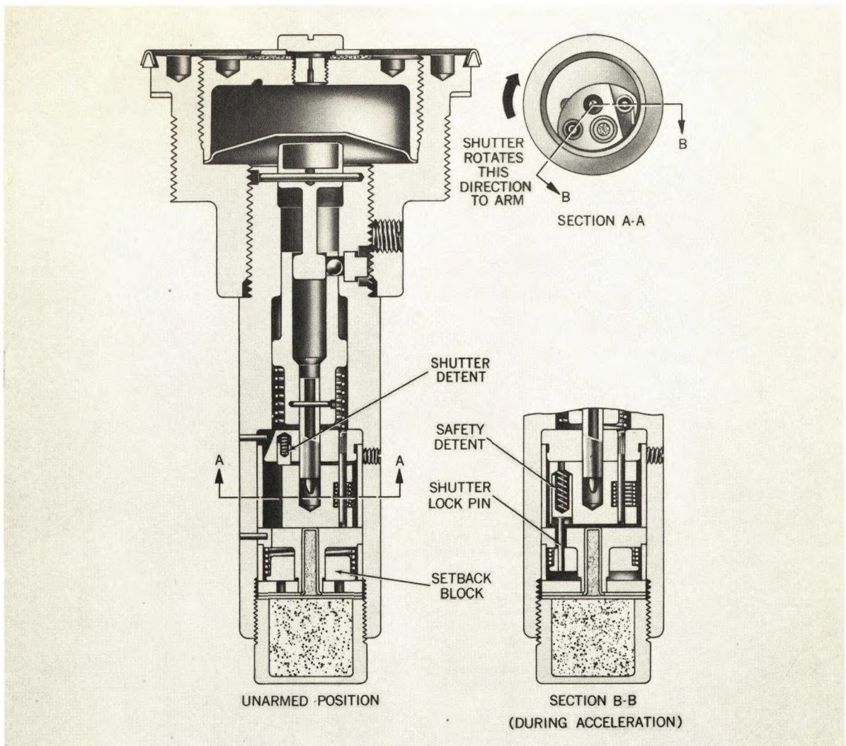
Figure 4-13. Base Fuze Mk 164 Mod 0, Cross Section, Unarmed Position.
