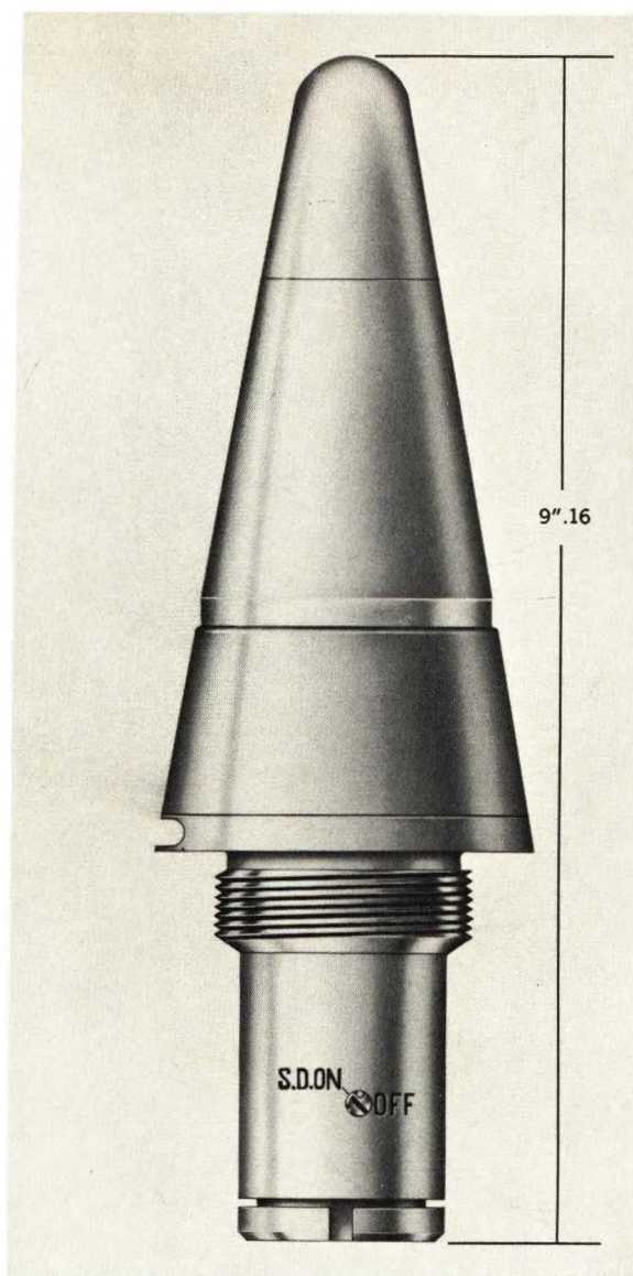
Figure 4-4. Nose (VT) Rocket Fuze T2061, External View.
