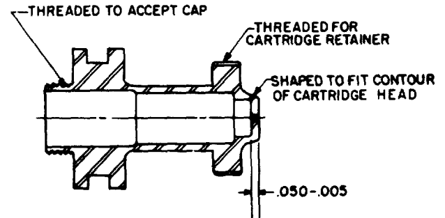
Figure 85. Firing-pin housing for initiator.
