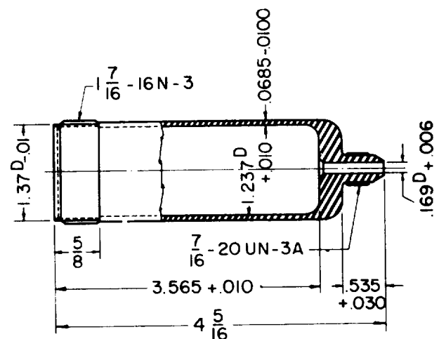
Figure 80. Initiator chamber.
