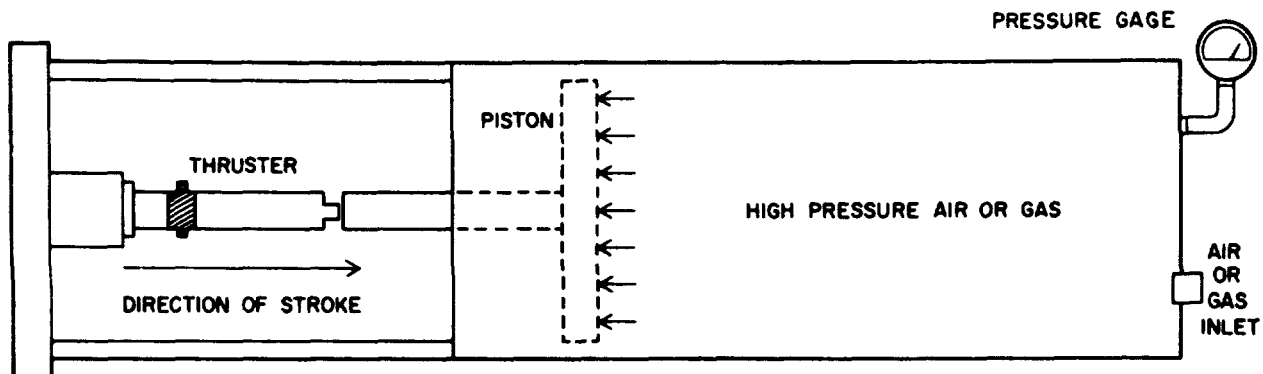
Figure 98. Pressure cylinder.
