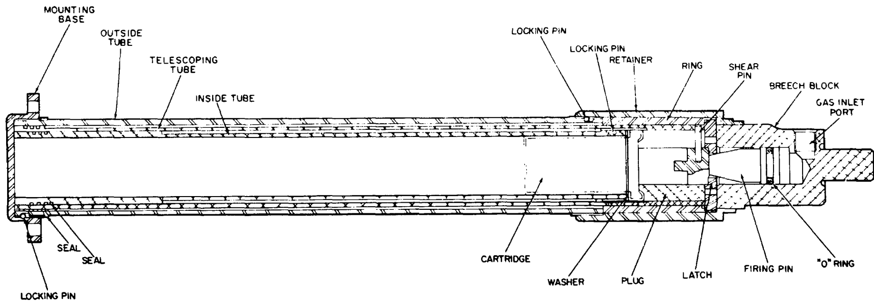
Figure 4. Typical remover.
