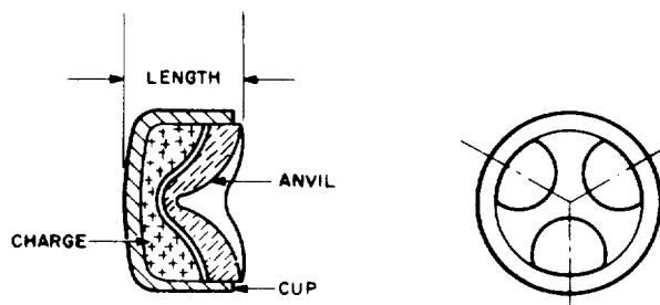
Figure 28. Percussion primer.
