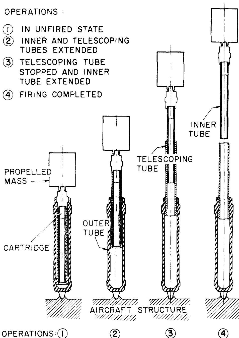
Figure 3. Operation of a conventional catapult.
