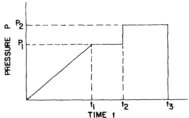
Figure 42. "Ideal" Pressure vs time curve.
