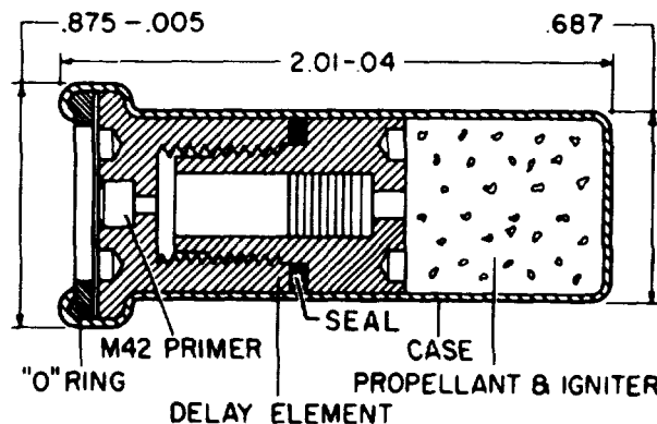
Figure 78. Initiator cartridge.
