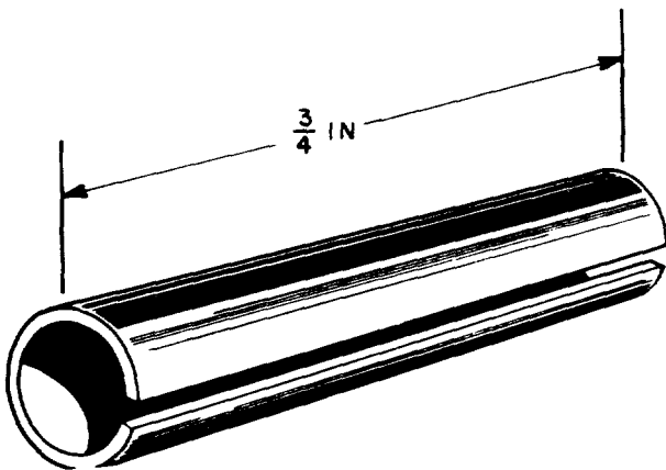
Figure 38. Spring pin.
