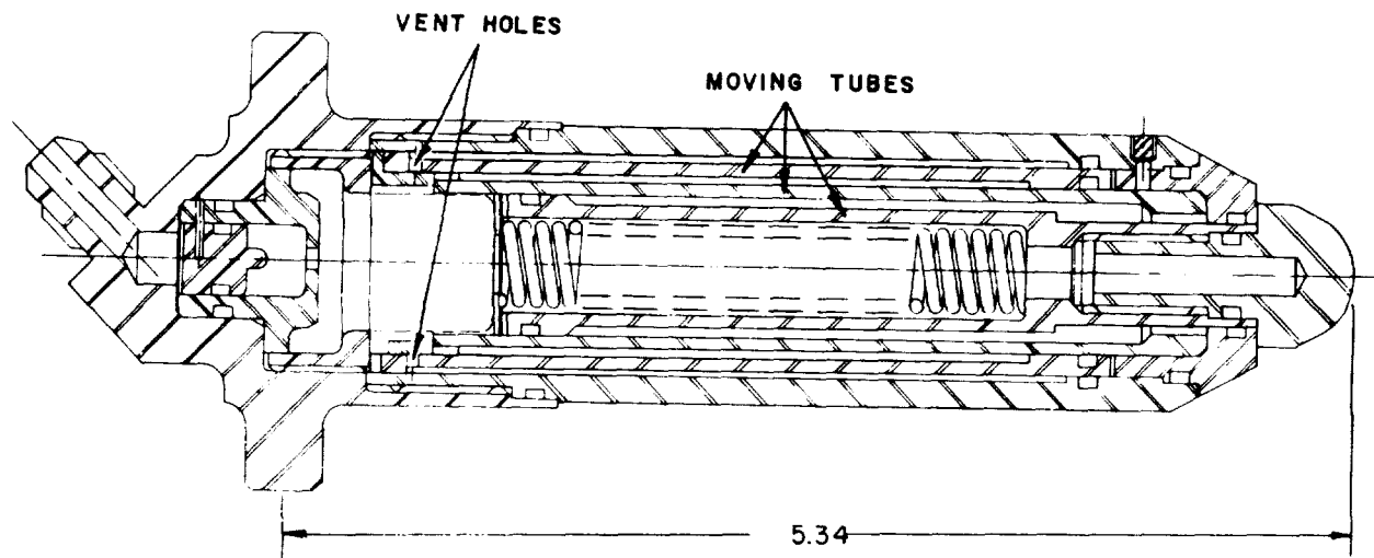
Figure 25. T28 Thruster.
