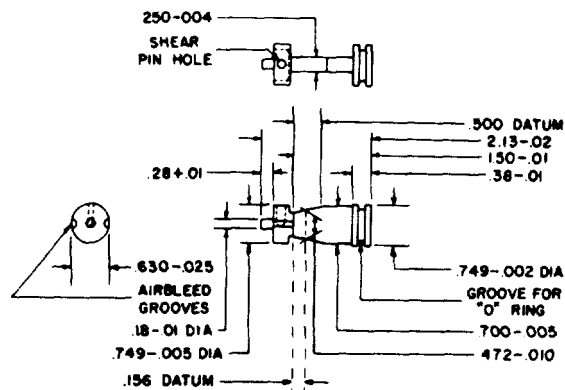
Figure 62. Firing pin for catapult.
