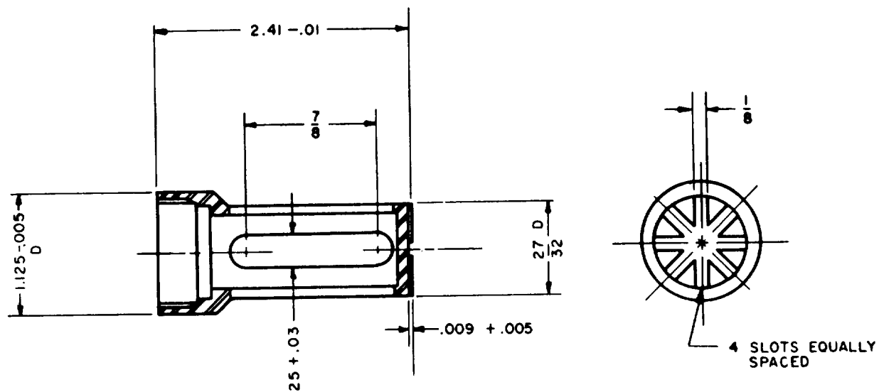
Figure 79. Cartridge retainer.
