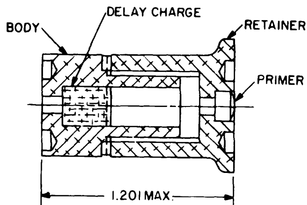
Figure 77. Delay element.
