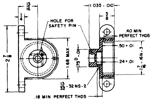
Figure 81. Initiator cap.
