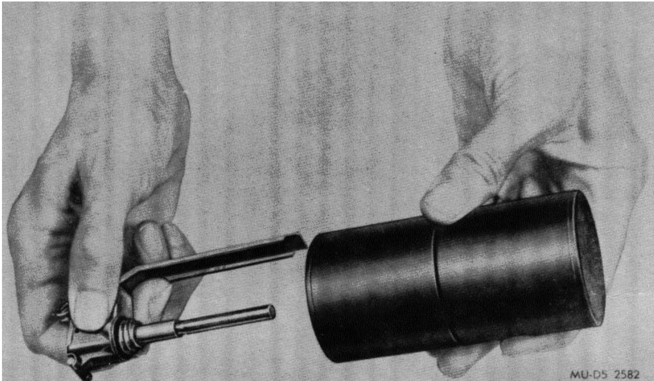
Figure 2-7. Screwing offensive grenade body onto fuze.
