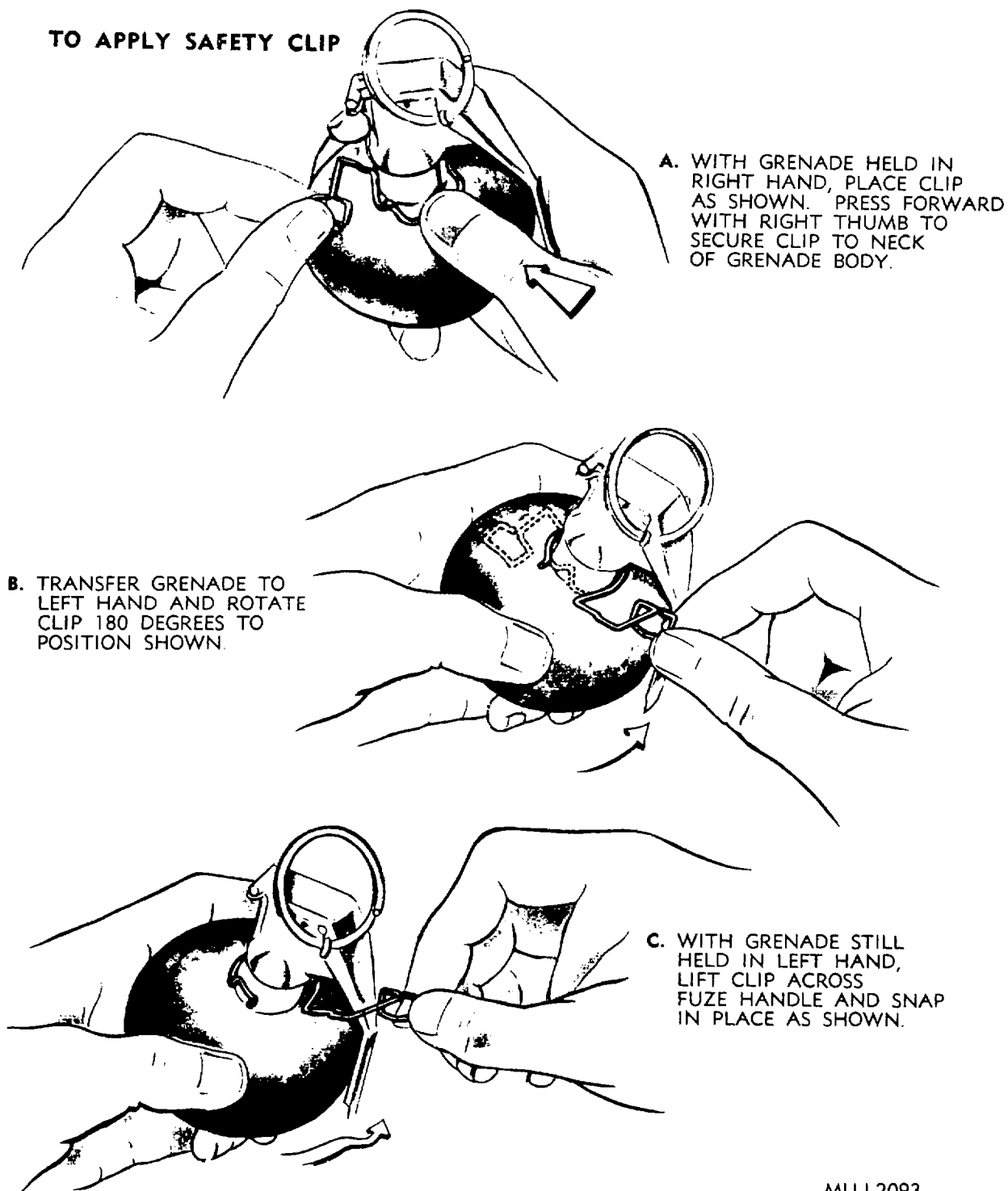
Figure 2-3. Assembly of safety clip to grenade M69.
