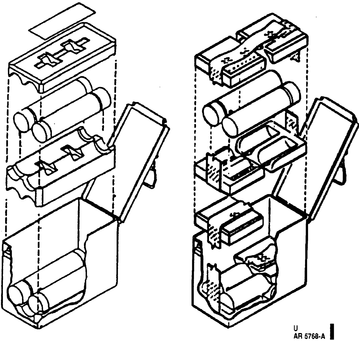
Figure 3-3.2. IR and simulant grenade boxes and packing.
