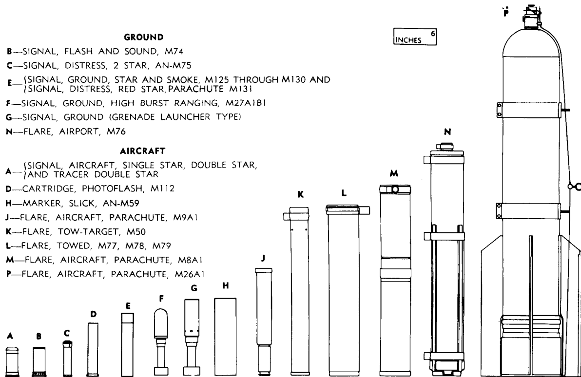
Figure 134. Military pyrotechnics—types and comparative sizes.
