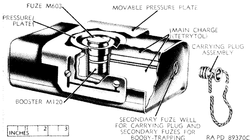
Figure 178. Mine, antitank, HE, light, M7A2, and fuze, mine, antitank, M603 (T17E2).
