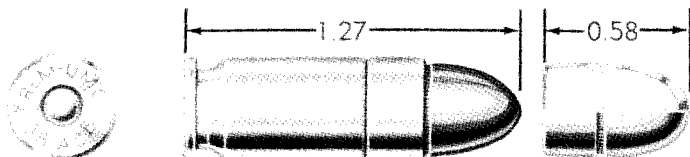
CARTRIDGE, BALL, CAL. .38, SUPER AUTOMATIC COLT, 130-GRAIN BULLET, METAL JACKET
