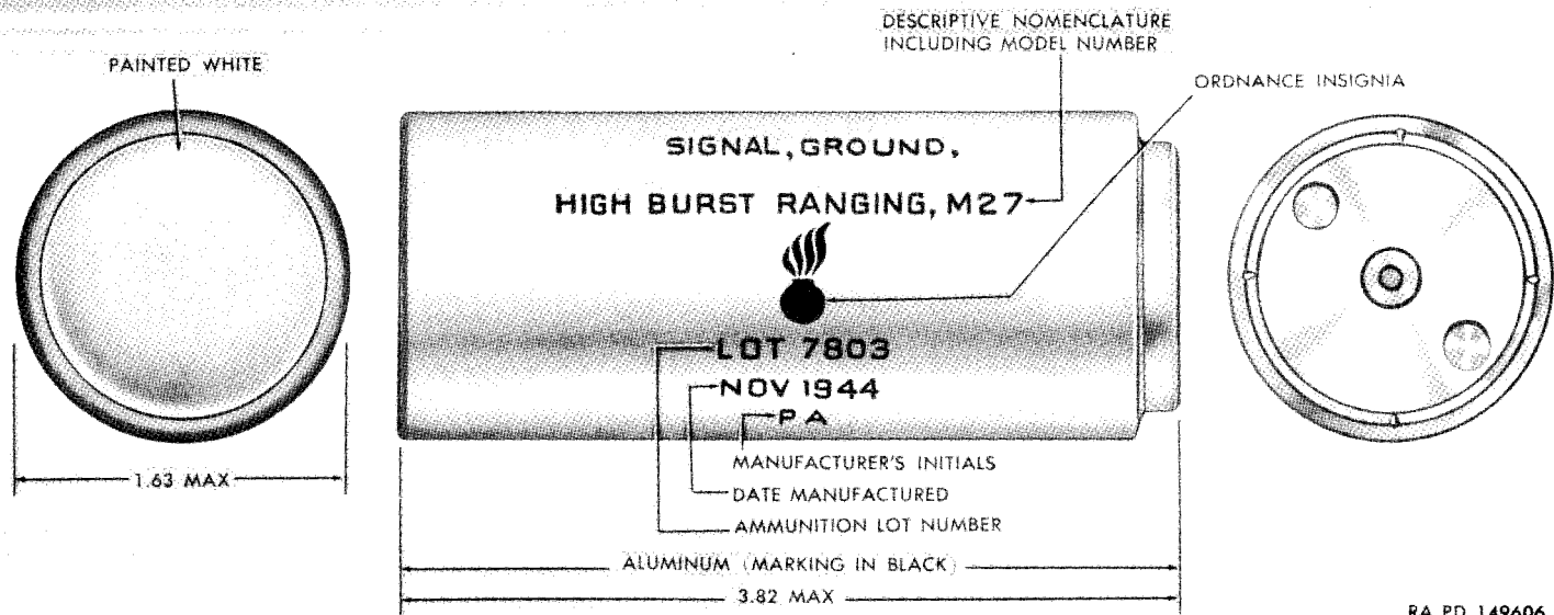
Figure 150. Signal, ground, high burst ranging, M27.
