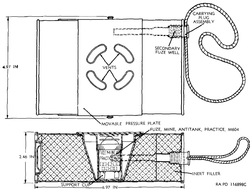
Figure 181. Mine, antitank, light, practice, M10 (T9), with fuze, mine, antitank, practice, M604.
