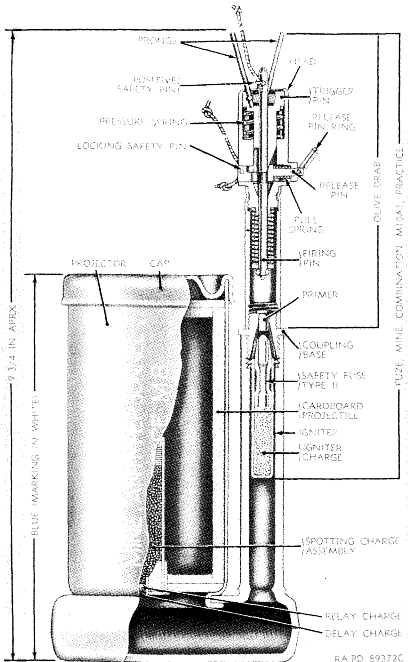
Figure 175. Mine, antipersonnel, practice, M8 (T4), and fuze, mine, combination, M10 (T14) or M10A1, practice.
