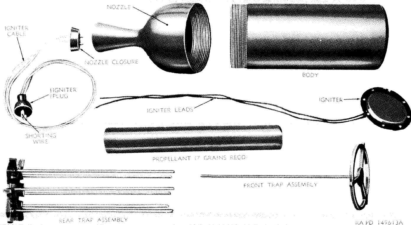
Figure 171. Components of a typical JATO.
