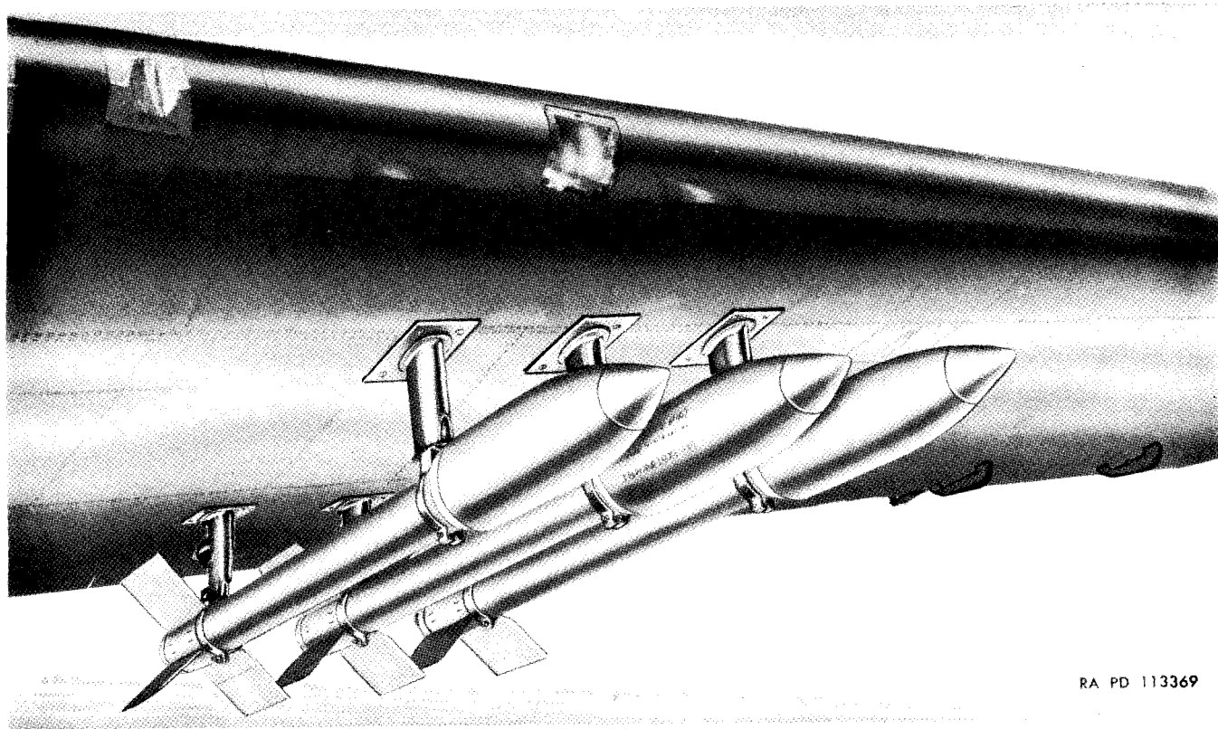
Figure 163. 5.0-inch aircraft rockets on Navy post launchers.
