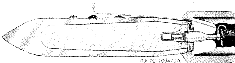
Figure 116. Armor-piercing bomb—section.
