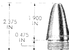
FUZE, DUMMY, M69, FOR 40-MM PRACTICE AND DRILL ROUNDS
