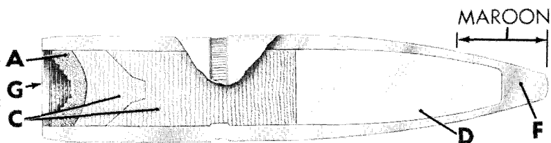
BULLET, TRACER, CAL. .50, M17
