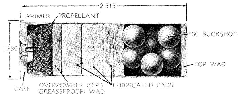
Figure 55. 12-gage paper shotgun shell—sectioned.
