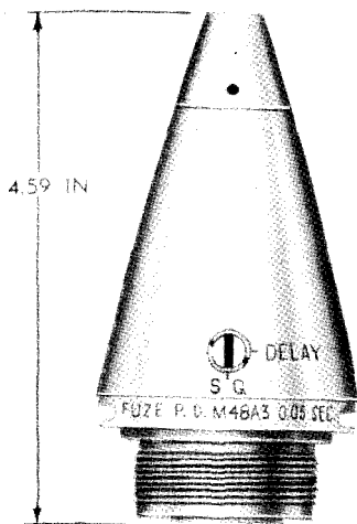
M48A3 SQ AND 0.05-SEC DELAY IMPACT
