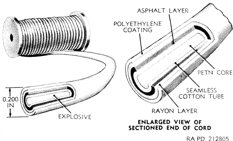
Figure 199. Cord, detonating, waterproof.
