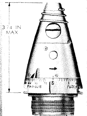
M501A1 MECHANICAL TIME AND SUPERQUICK (MTSQ)
