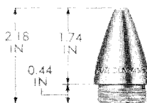
FUZE, DUMMY, M50, FOR 37-MM PRACTICE AND DRILL ROUNDS
