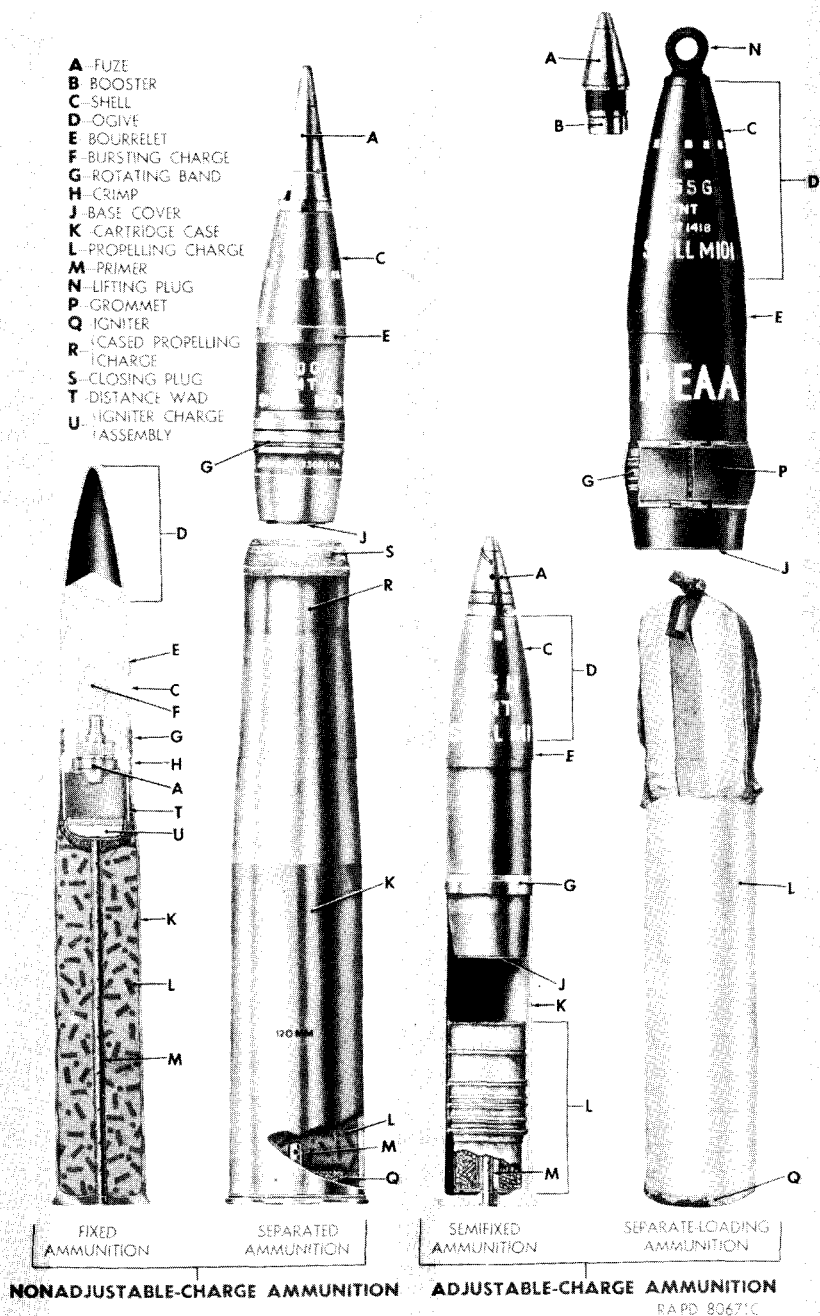
Figure 76. Types of complete rounds of artillery ammunition.
