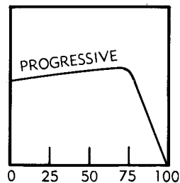
Figure 23. Comparative burning rates of different shaped propellant grains.
