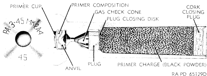
Figure 94. Percussion primer Mk 2A4—for separate-loading rounds.
