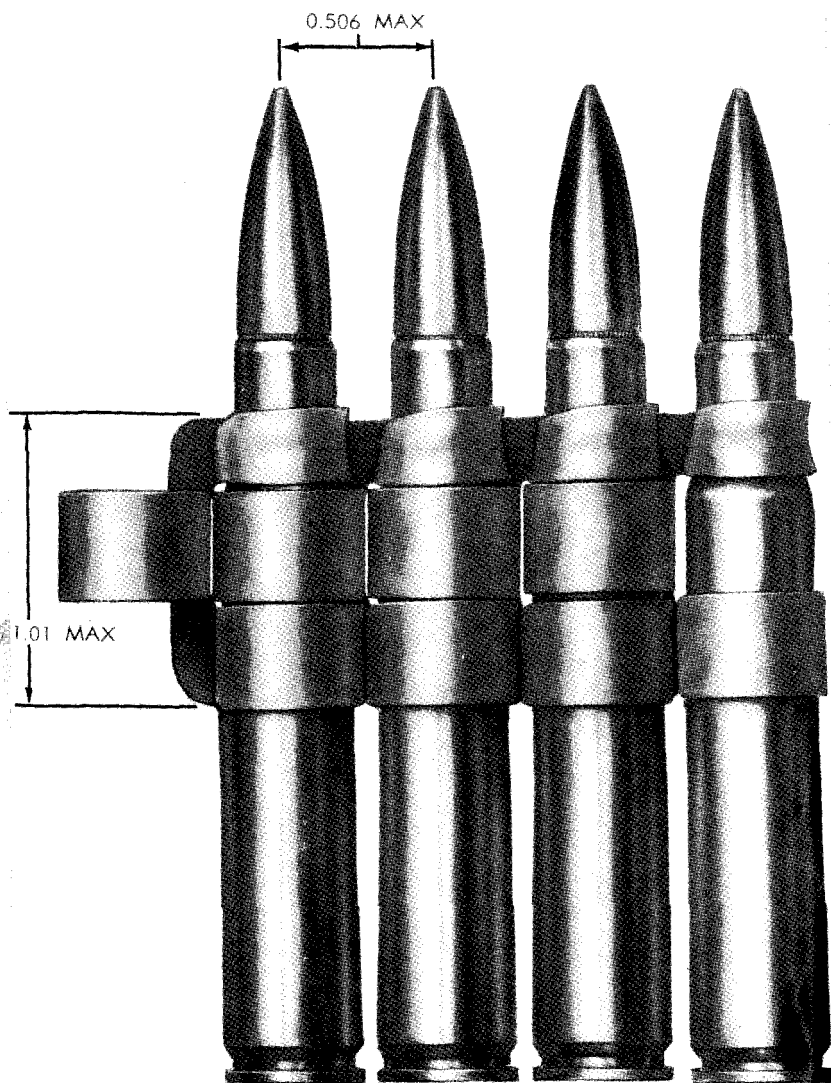
Figure 47. Section of metallic link belt of caliber .30 cartridges.
