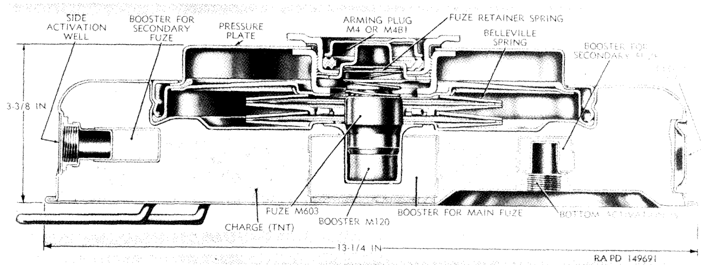
Figure 177. Mine, antitank, HE, heavy, M6A2, and fuze, mine, AT, M603 (T17E2).
