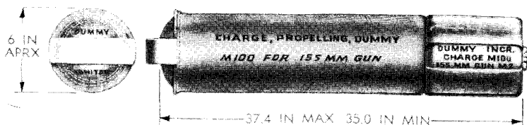
D-TYPICAL SEPARATE-LOADING DUMMY PROPELLING CHARGE
