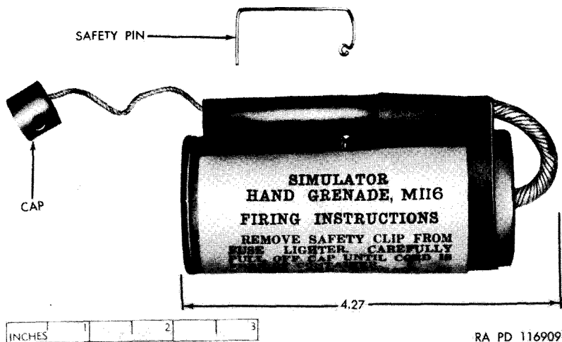
Figure 70. Simulator, hand grenade, M116 (T79).
