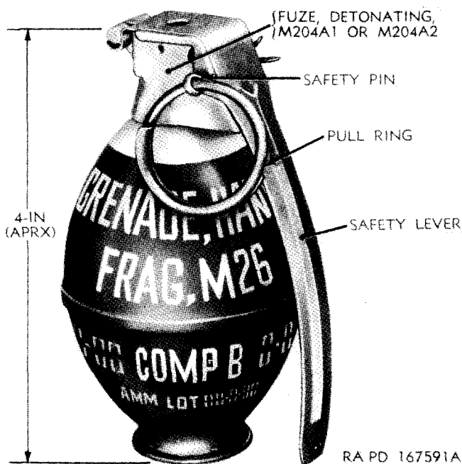
Figure 67. Grenade, hand, fragmentation, M26 (T38E1) fuzed with fuze M204A1 or M204A2.
