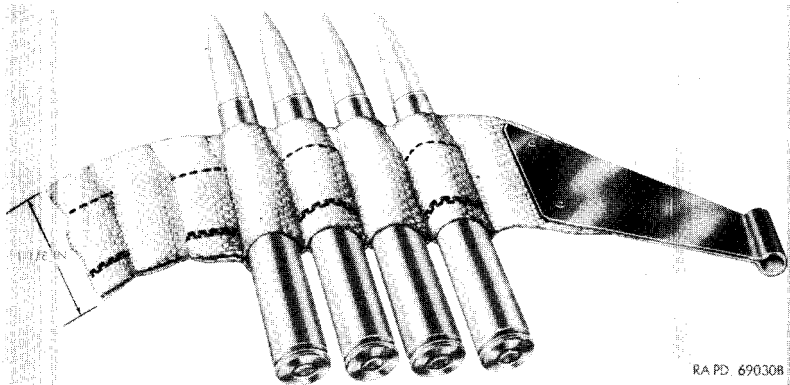
Figure 50. Section of 250-round web belt, caliber .30 M1917.
