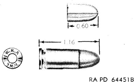
Figure 42. 9-mm ball cartridge.
