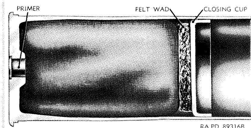
Figure 101. Blank ammunition for 75-mm guns and howitzers.
