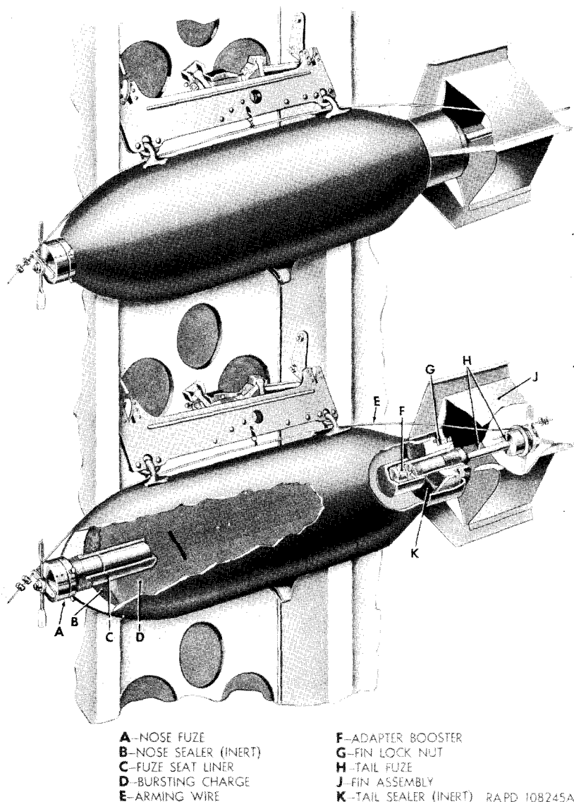
Figure 112. The complete round in bomb bay.
