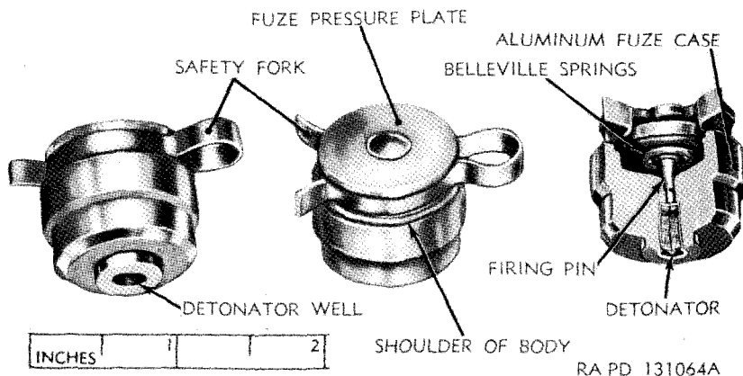
Figure 182. Fuze, mine, antitank, M603 (T17E2)—showing bottom, top, and cross section.
