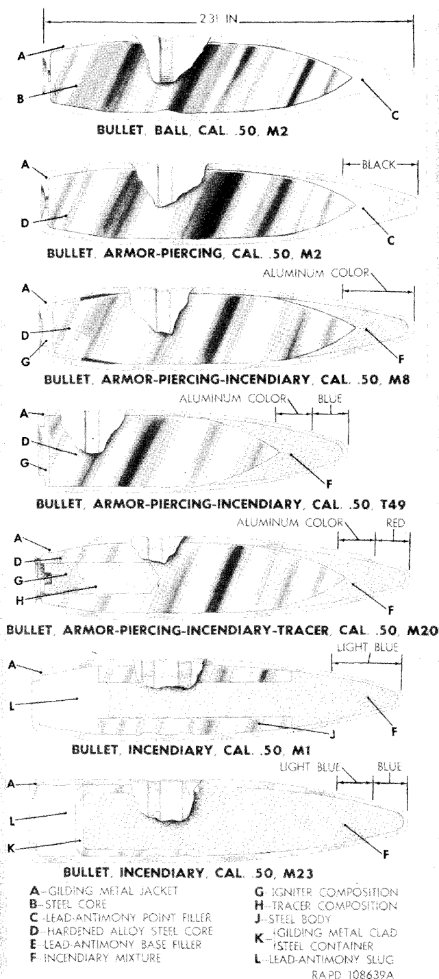
Figure 38. Caliber .50 bullets—sectioned.
