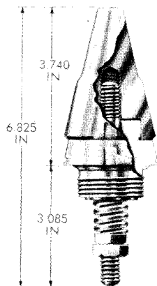
FUZE, DUMMY, M80, FOR 90-MM DRILL AND PRACTICE ROUNDS
