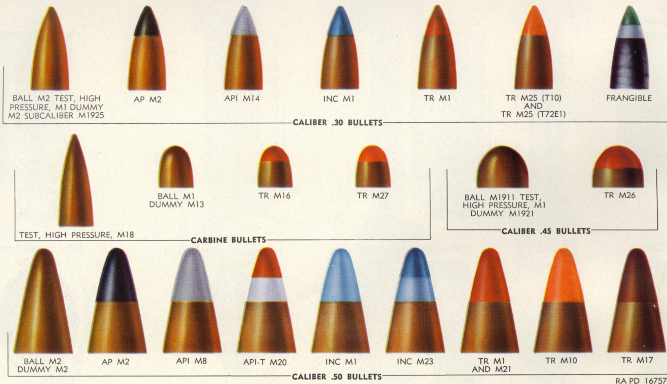
Figure 1. Color identification of bullets of small arm cartridges.
