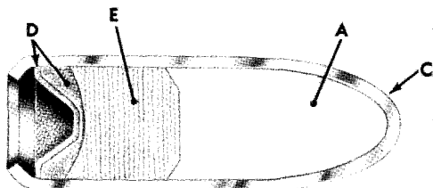
BULLET, TRACER, CARBINE, CAL. .30, M27 (T43)
