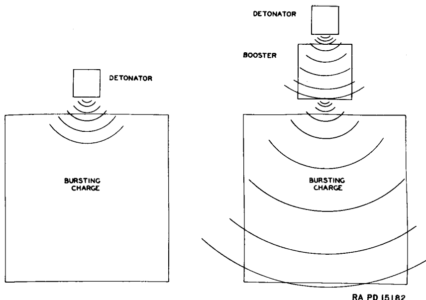
Figure 26. Detonating wave amplified by the use of a booster.
