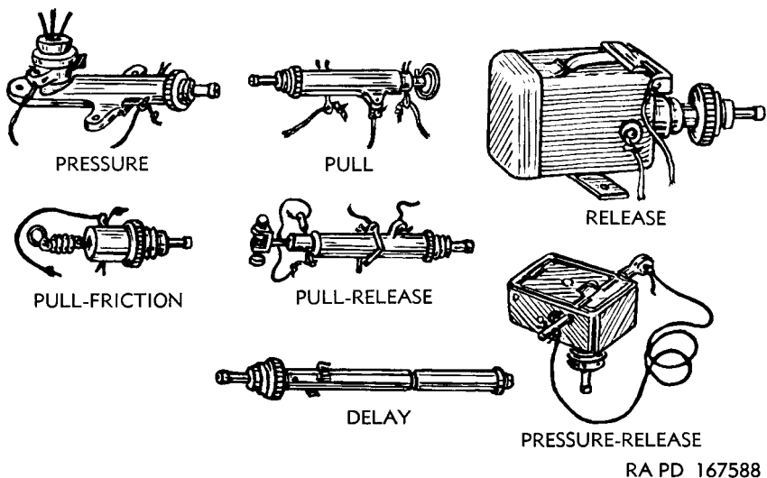
Figure 200. Firing devices.
