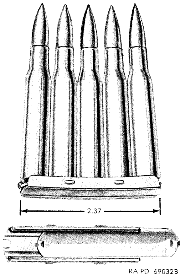
Figure 51. Caliber .30 cartridges in 5-round clip.
