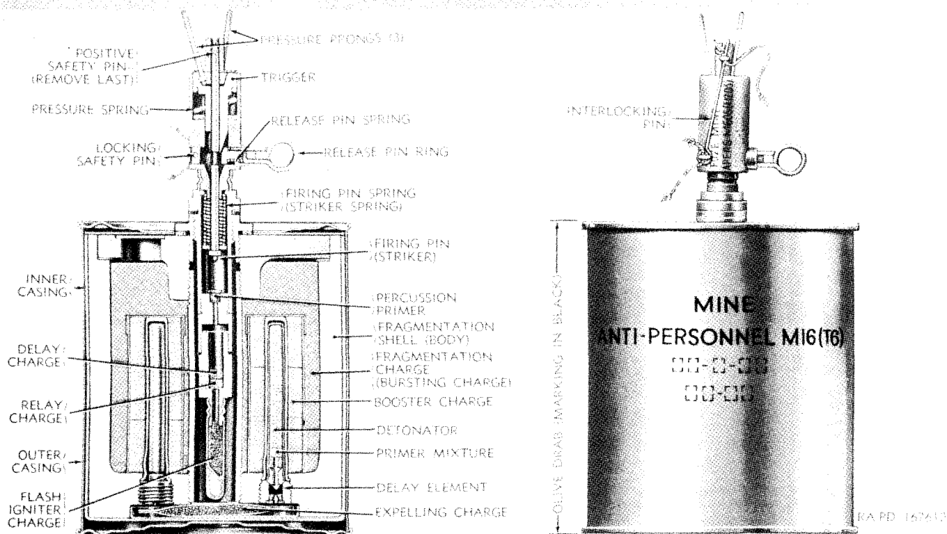
Figure 173. Mine, antipersonnel, M16, and fuze, mine, antipersonnel, M605.
