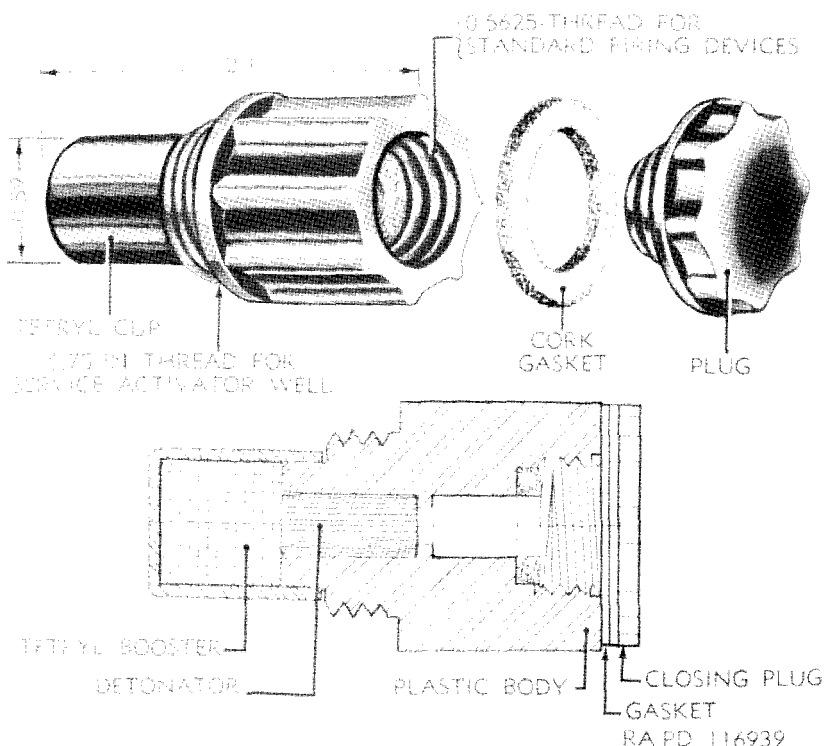
Figure 184. Activator, M1.
