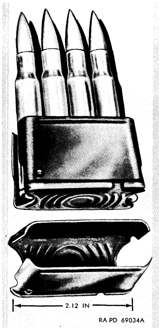
Figure 52. Caliber .30 cartridges in 8-round clip.
