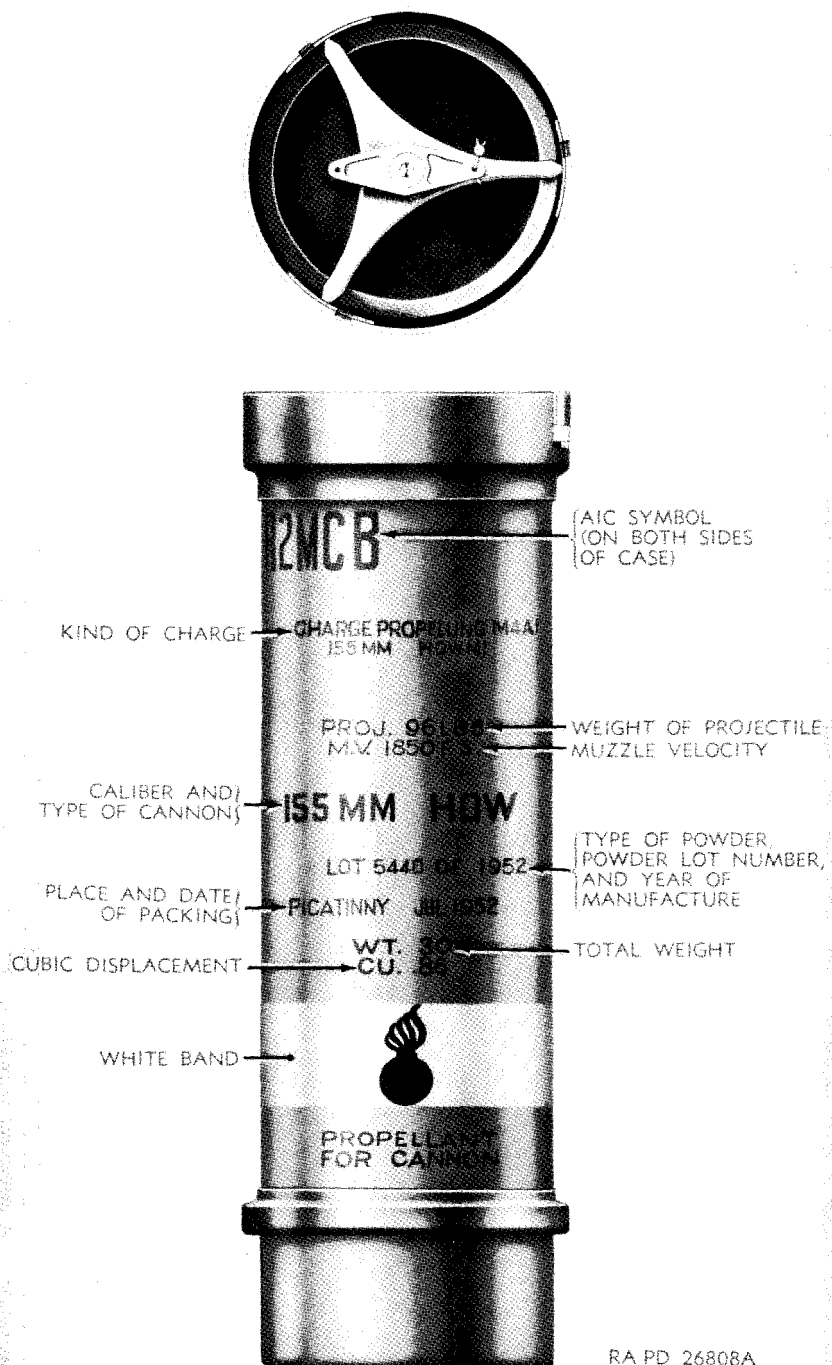
Figure 109. Metal container for propelling charge.
