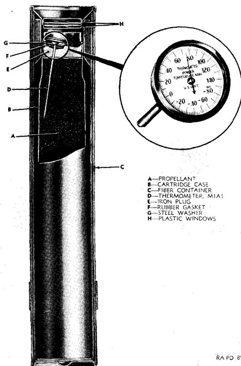
Figure 102. Propellant temperature indicator with thermometer.
