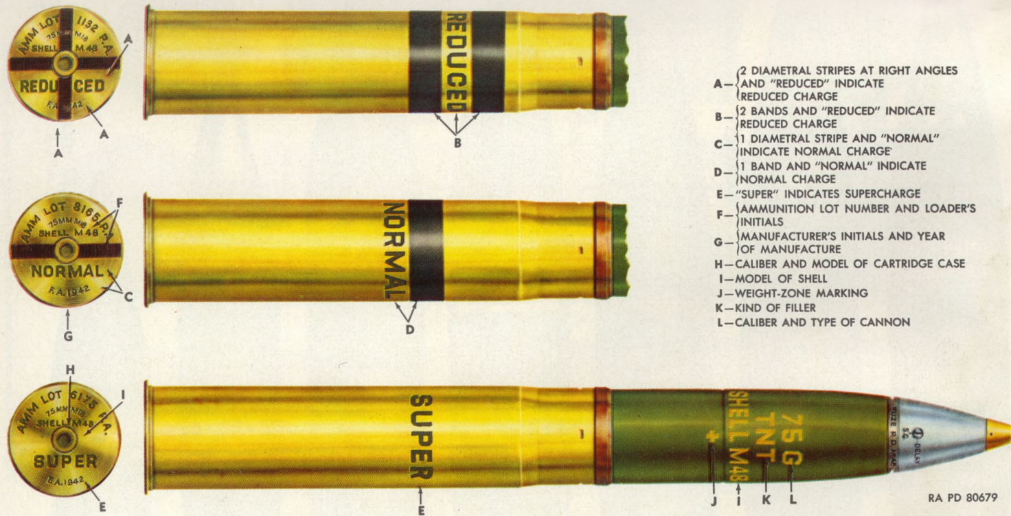
Figure 7 Color identification and typical marking of reduced, normal, and supercharge artillery ammunition.
