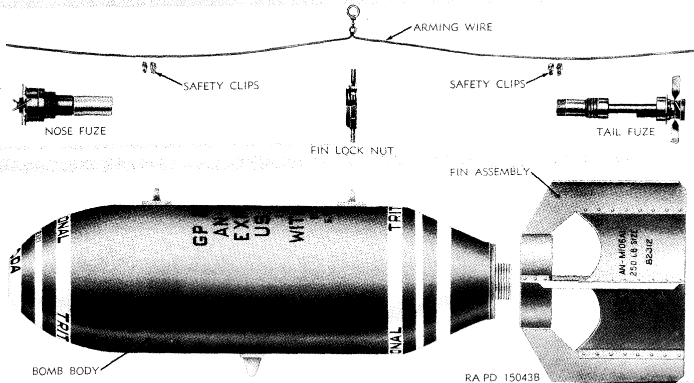
Figure 110. Components of bombs.
