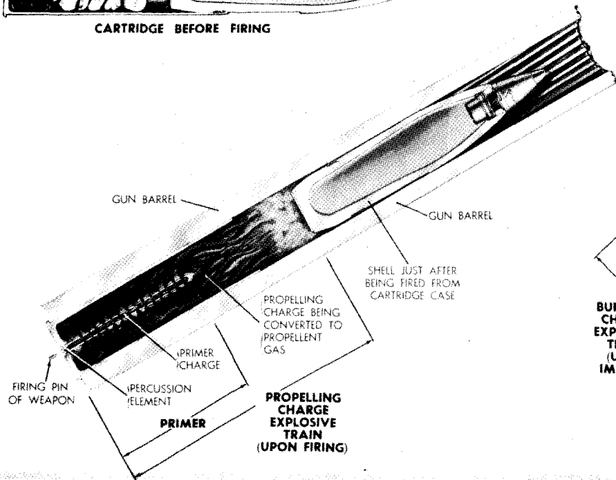
Figure 25. Explosive trains—artillery ammunition.
