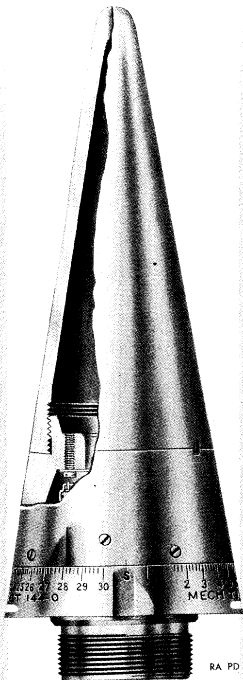
Figure 91. Point-detonating mechanical-time fuze for separated ammunition.
