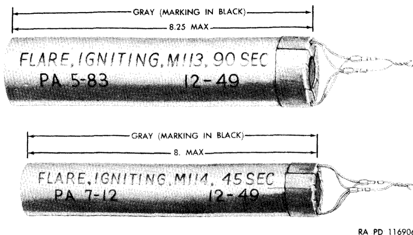
Figure 142. Flare, igniting, M113, 90-second, and flare, igniting, M114, 45-second.
