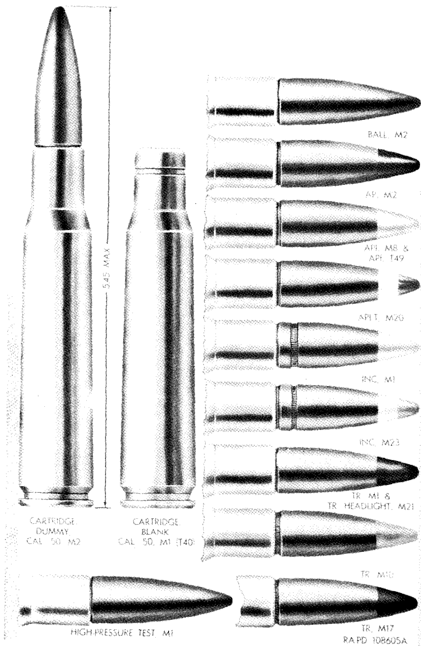
Figure 31. Caliber .50 cartridges.
