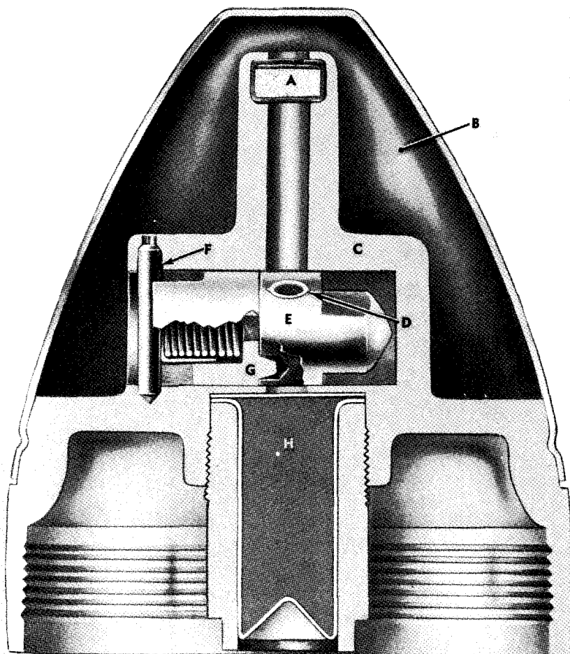
Figure 87. Point-initiating base-detonating (PIBD) fuze M90A1, for 57-mm rifle shell.
