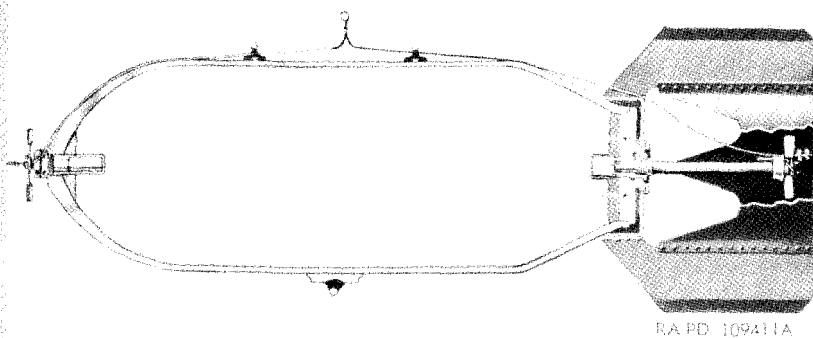
Figure 114. General-purpose bomb—section.
