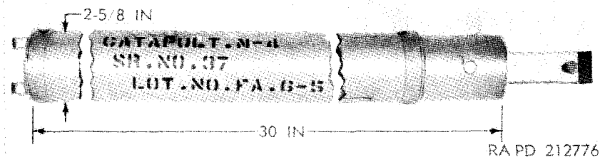
Figure 213. Catapult M4.
