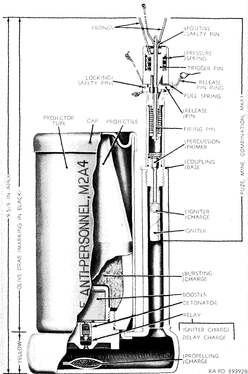
Figure 172. Mine, antipersonnel, M2A4, and fuze, mine, combination, M6A1.
