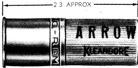
SHELL, SHOTGUN, 12-GAGE, PAPER, LOADED WITH SMOKELESS POWDER AND #00 BUCKSHOT
