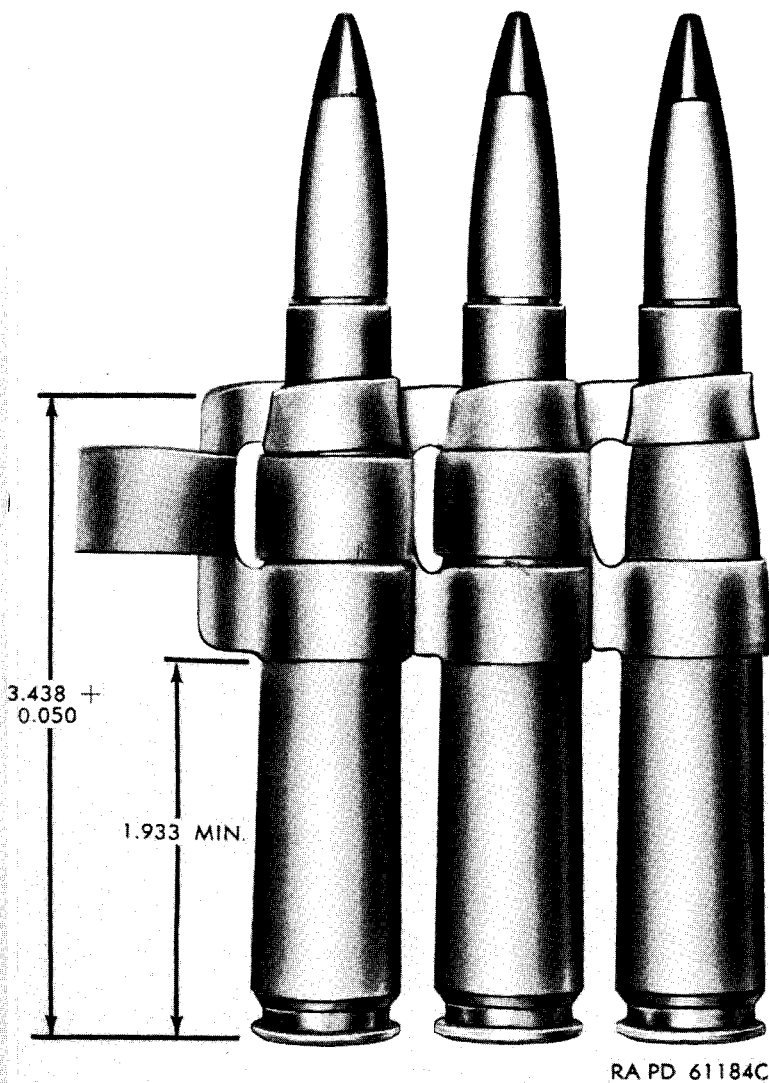
Figure 48. Section of metallic link belt of caliber .50 cartridges.
