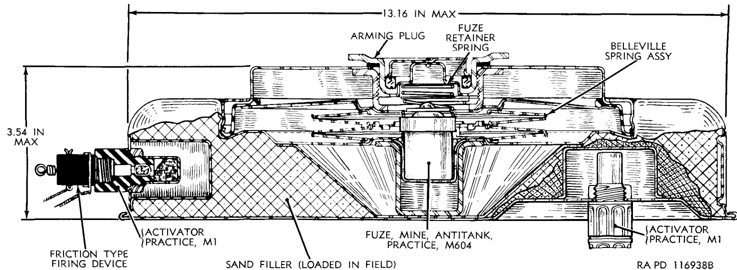
Figure 180. Mine, antitank, heavy, practice, M12 (T8E1), with fuze, mine, antitank practice, M604.
