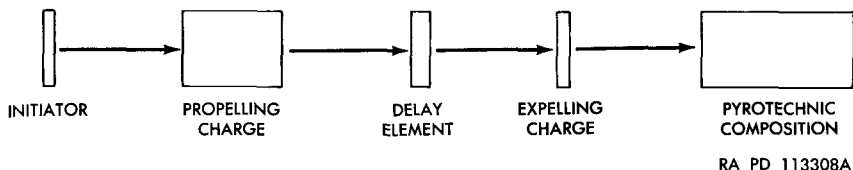
Figure 135. Representative ignition train for pyrotechnics.
