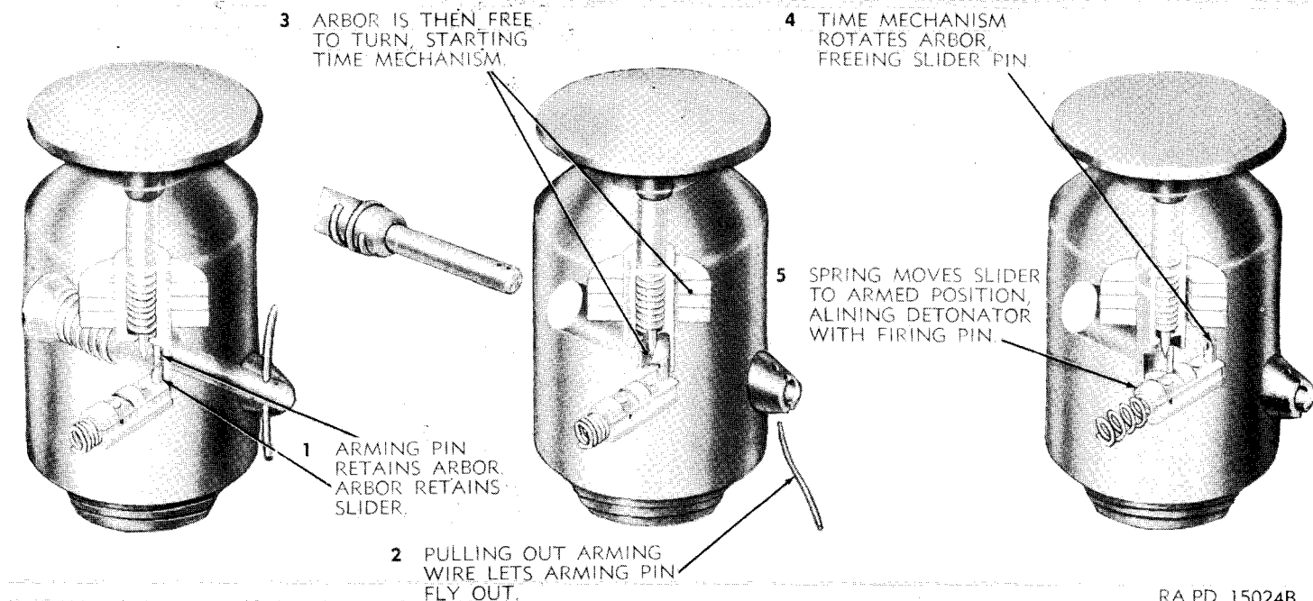
Figure 126. Method of arming—arming-pin-type fuze.
