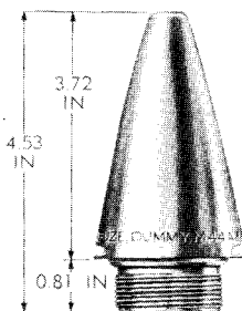
FUZE, DUMMY, M44A2, FOR 90-MM DRILL AND PRACTICE ROUNDS
