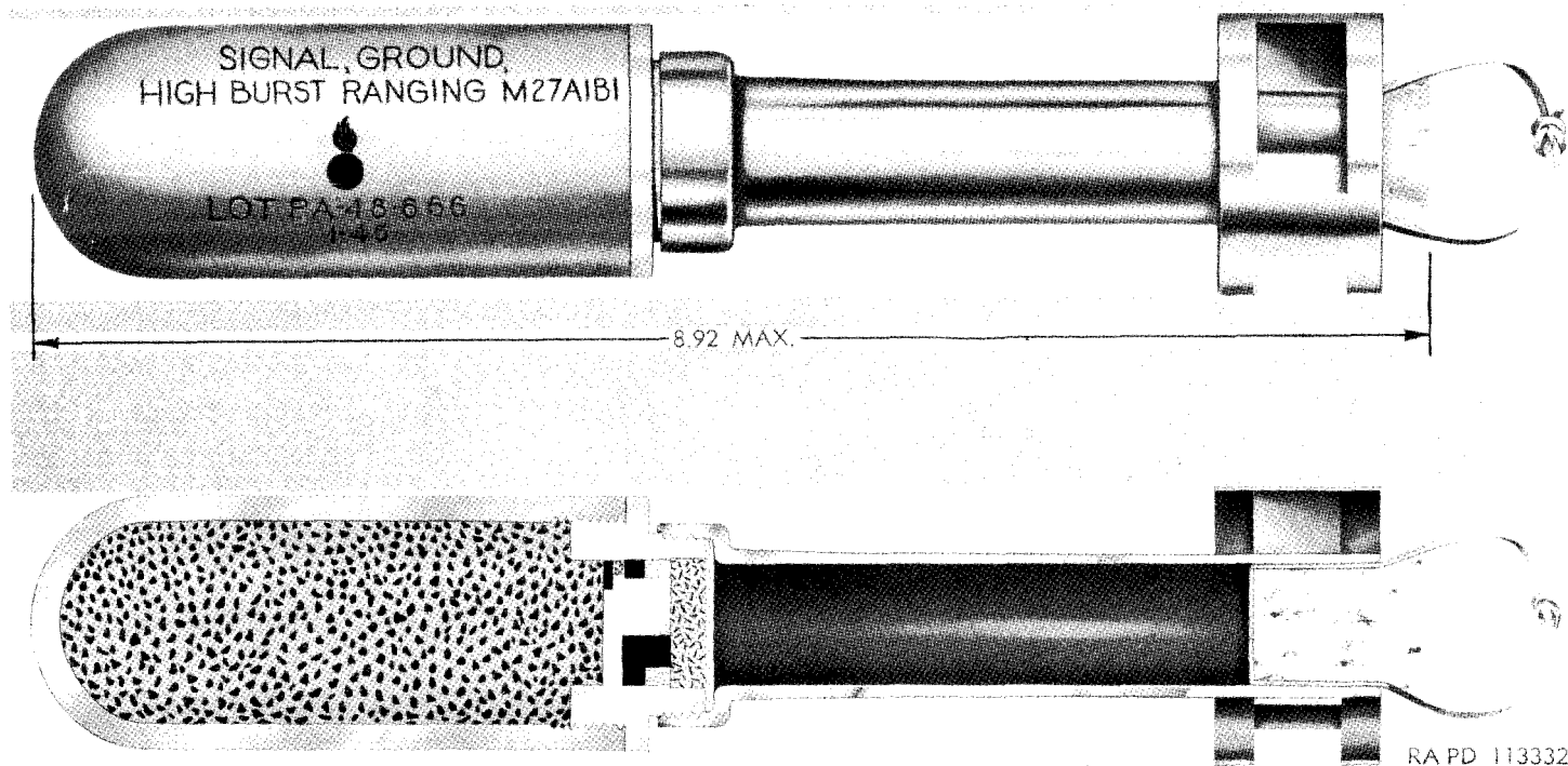
Figure 151. Signal, ground, high burst ranging, M27A1B1.
