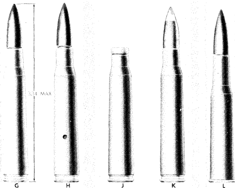
Figure 29. Caliber .30 cartridges.
