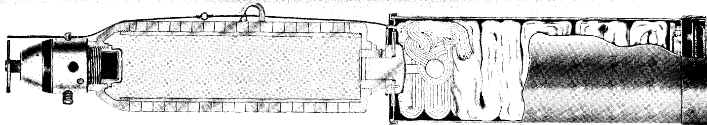
FRAGMENTATION BOMB (PARACHUTE TYPE)
