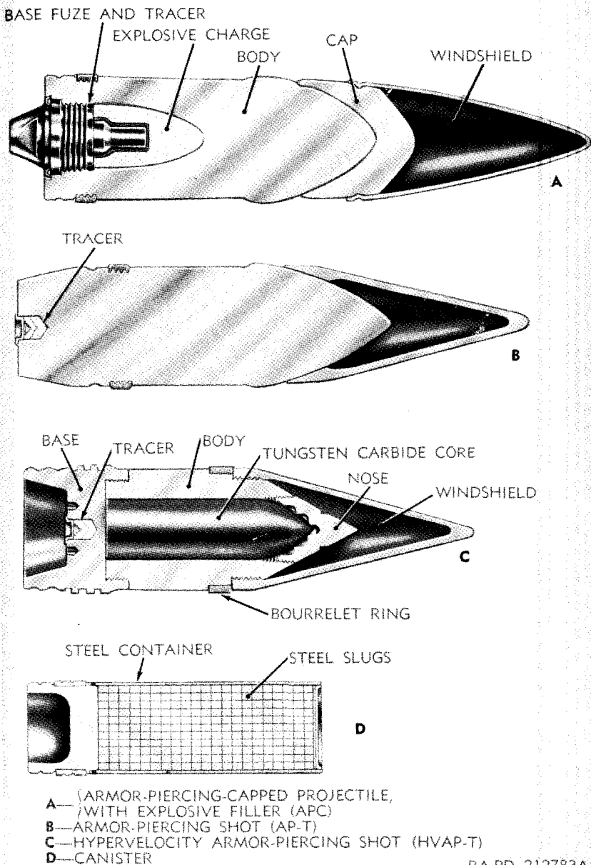
Figure 81. Typical armor-piercing and canister projectiles.
