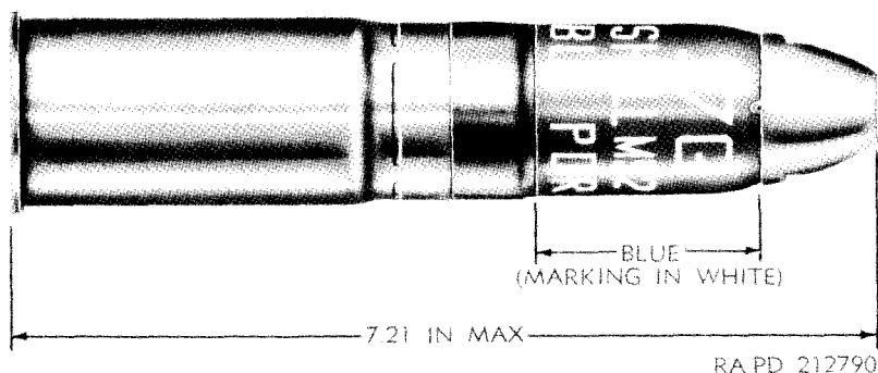
Figure 100. Target-practice shell for 37-mm subcaliber gun.
