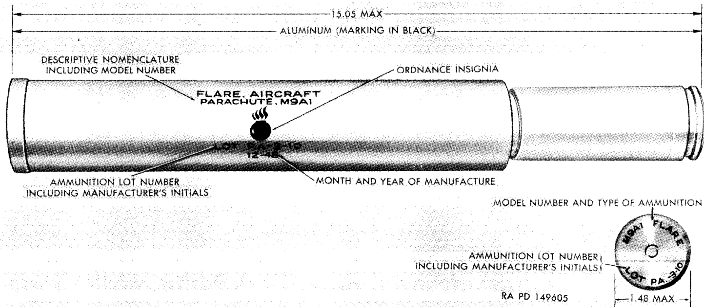
Figure 136. Flare, aircraft, parachute, M9A1.
