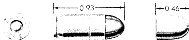
CARTRIDGE, BALL, AUTOMATIC PISTOL, CAL. .380, 95-GRAIN BULLET (9-MM SHORT)
