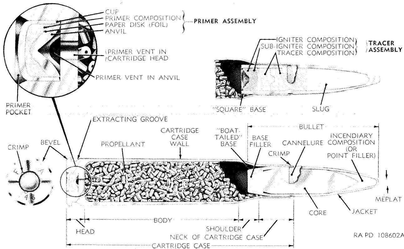
Figure 33. Cartridge terminology.
