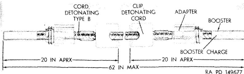
Figure 208. Priming assembly, demolition, M15.
