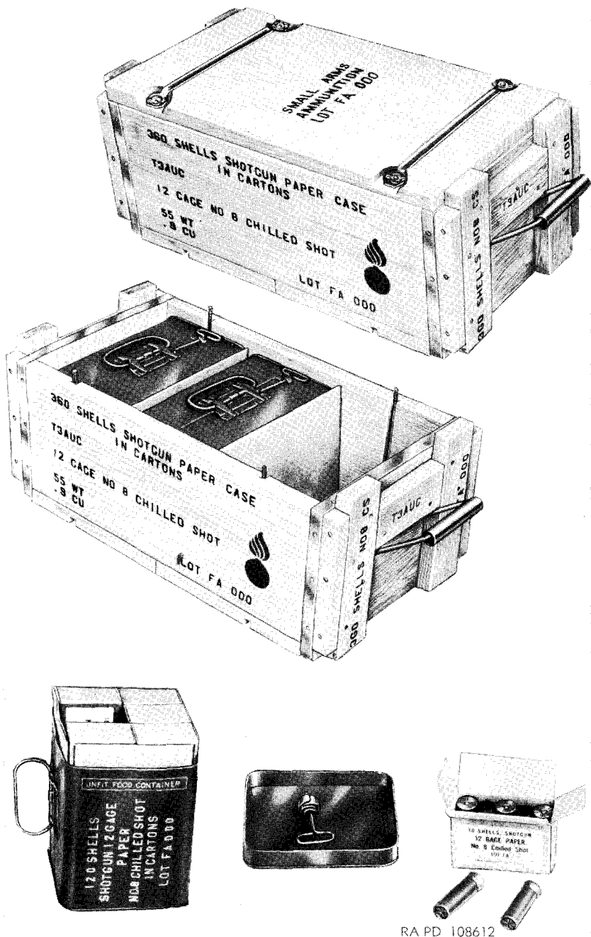
Figure 66. 12-gauge paper shotgun shell in cartons, in metal can M10, and in box M15.
