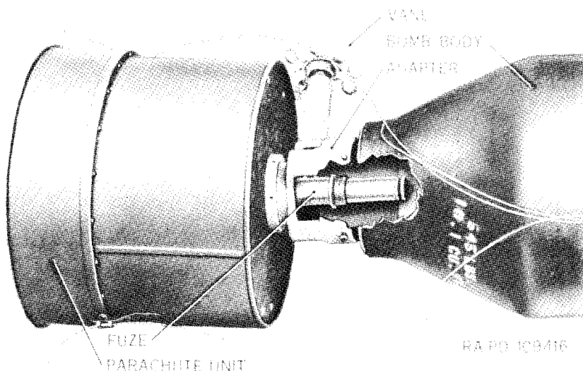
Figure 132. Antiricochet device assembled to bomb—sectioned.
