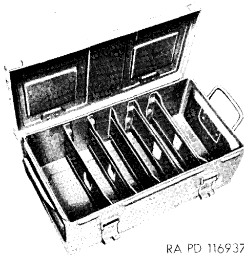
Figure 190. Metal packing box M156 for 8 mine, anti-tank, HE, M7A1, and 8 fuze, mine, antitank, M603, or 12 mine, antitank, light, practice, M10, without fuze.
