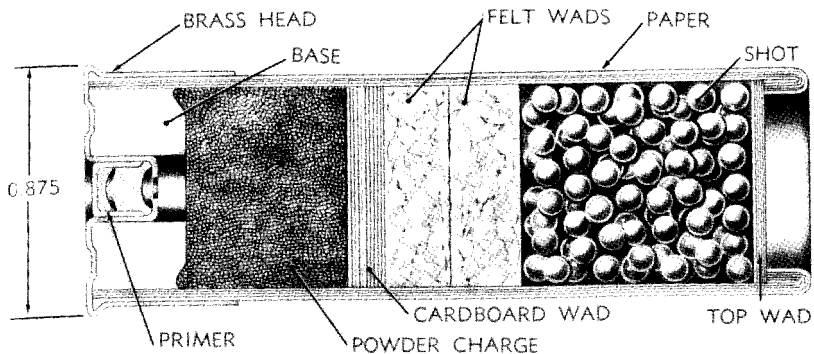
Figure 55. 12-gage paper shotgun shell—sectioned.
