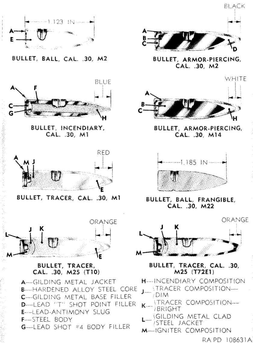
Figure 35. Caliber .30 bullets—sectioned.
