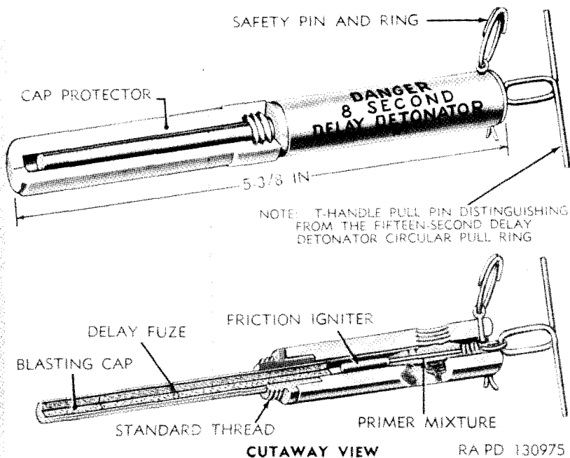
Figure 195. Detonator, 8-second delay, M2.
