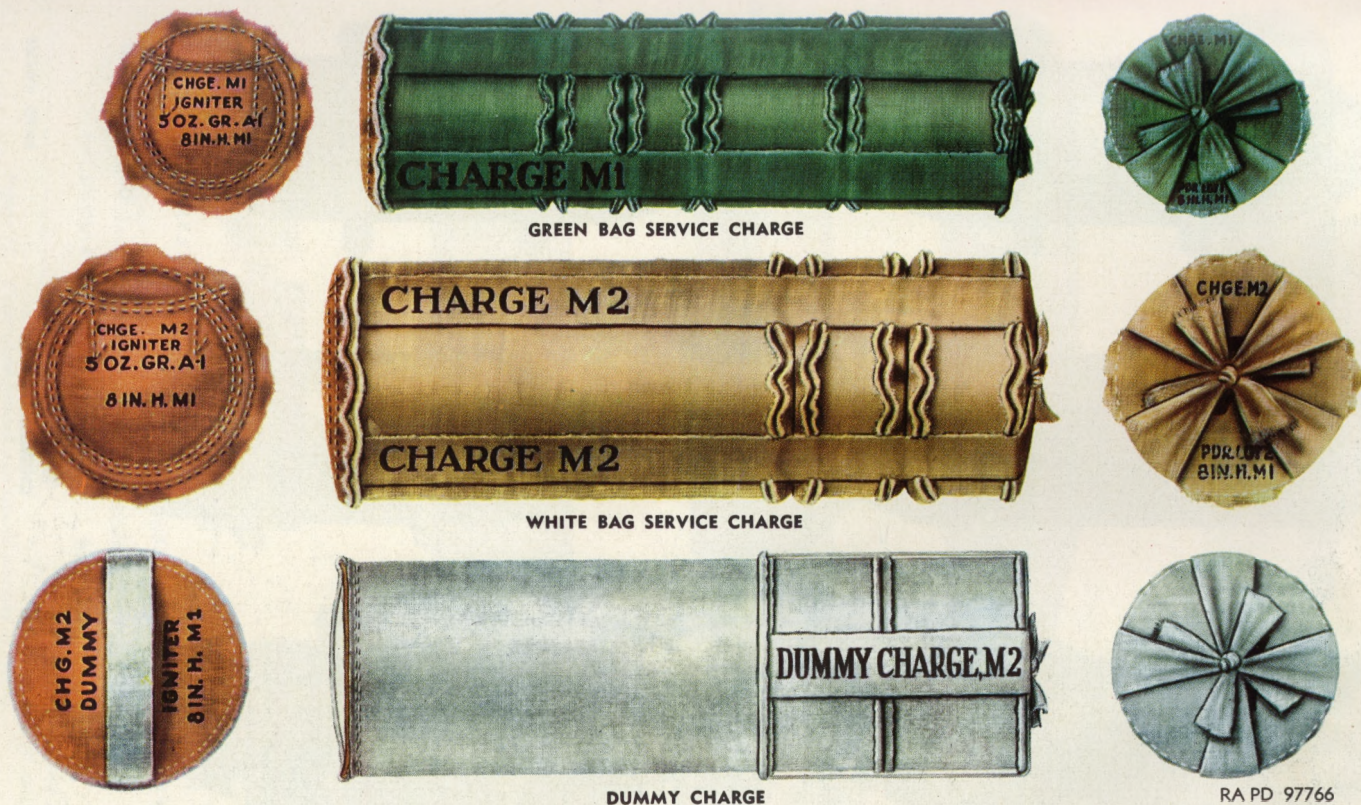
Figure 9. Color identification and typical marking of artillery propelling charges.
