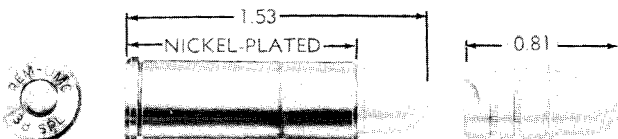
CARTRIDGE, BALL, REVOLVER, CAL. .38, SPECIAL, 200-GRAIN BULLET, NICKEL-PLATED CARTRIDGE CASE ("SUPER-POLICE")
