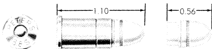
CARTRIDGE, BALL, REVOLVER, CAL. .38, SHORT COLT, 125- OR 130-GRAIN BULLET
