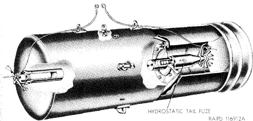
Figure 118. Depth bomb—section.
