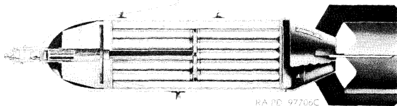
Figure 122. Target-identification bomb—section.
