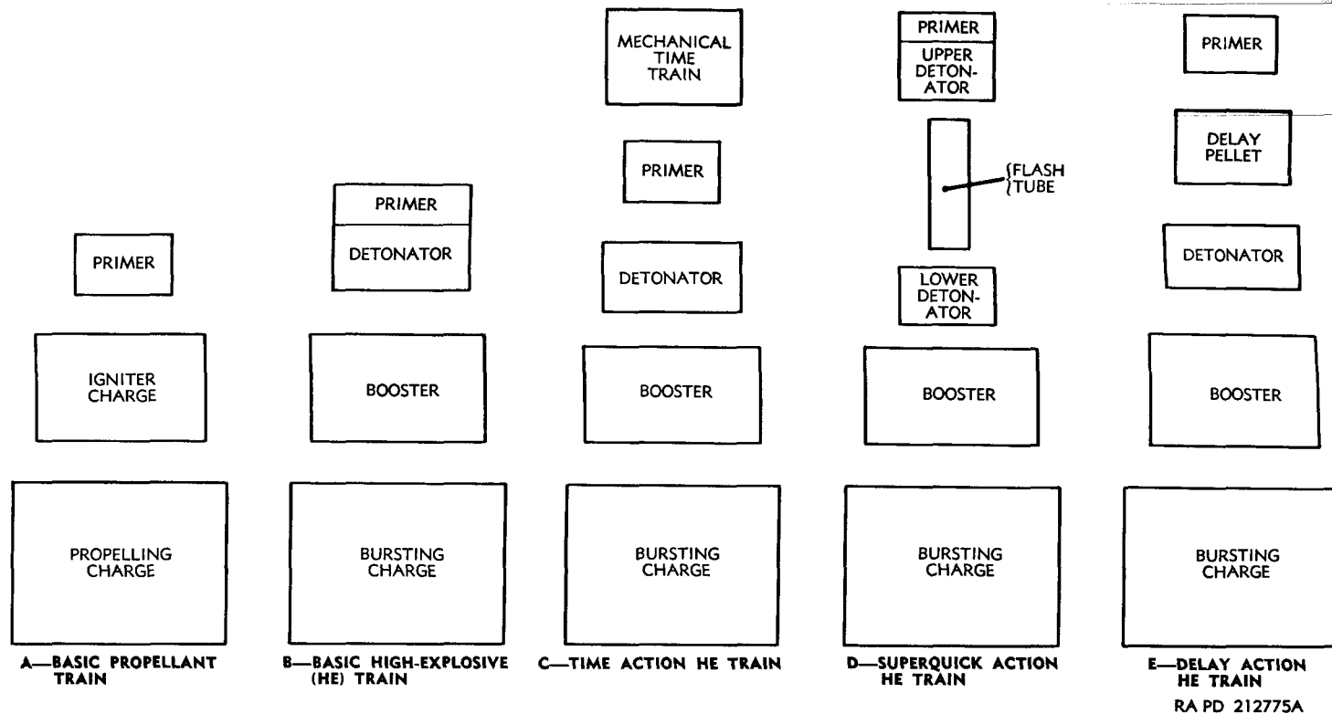
Figure 27. Schematic arrangement of components of explosive trains.
