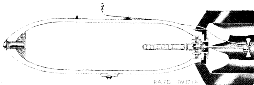
Figure 117. Semi-armor-piercing bomb—section.
