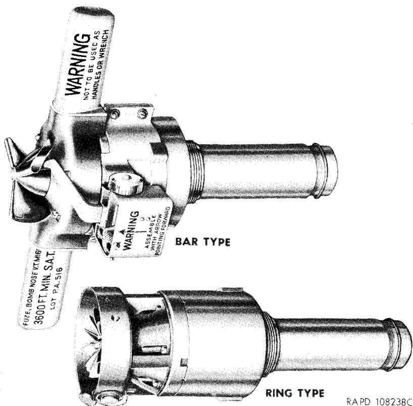
Figure 129. VT fuzes.
