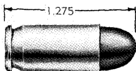
CARTRIDGE, BALL, CAL. .45, M1911
