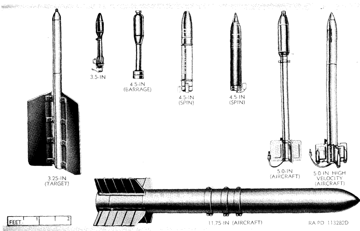
Figure 158. Representative types of rockets.
