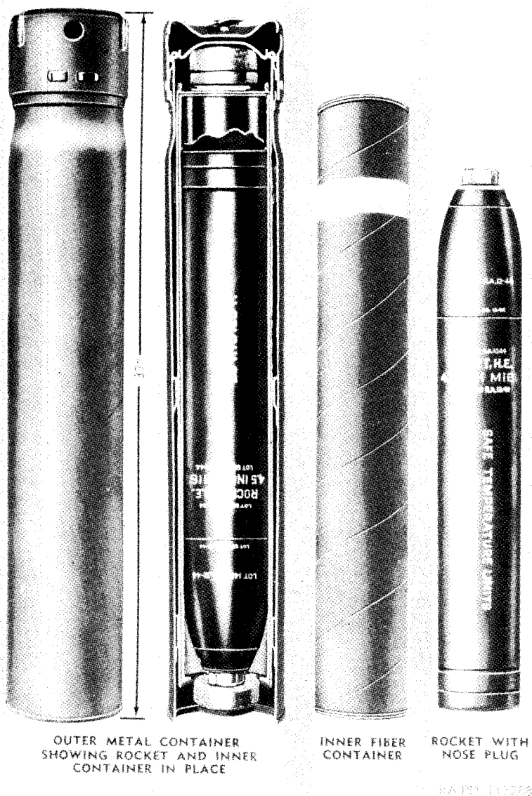
Figure 167. Packing—outer metal and inner fiber containers for 4.5-inch rocket.
