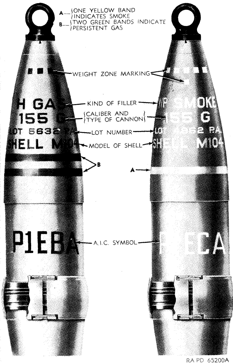
Figure 84. Chemical projectile.
