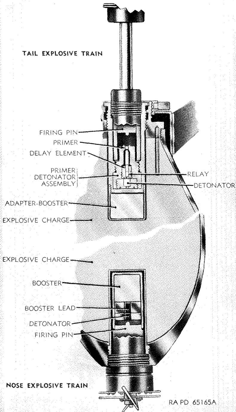
Figure 113. Explosive train.
