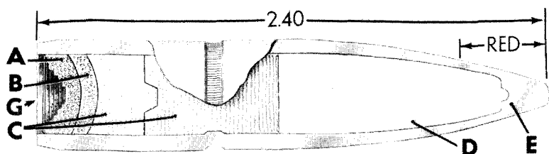
BULLET, TRACER, CAL. .50, M1
