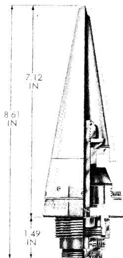
FUZE, DUMMY, M79, FOR 120-MM DUMMY PROJECTILES
