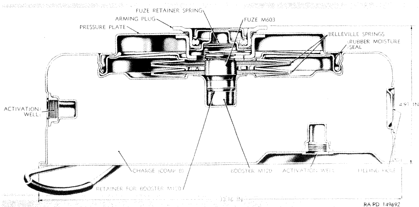
Figure 176. Mine, antitank, HE, heavy, M15 (T27)—cross section with fuze M603 installed.
