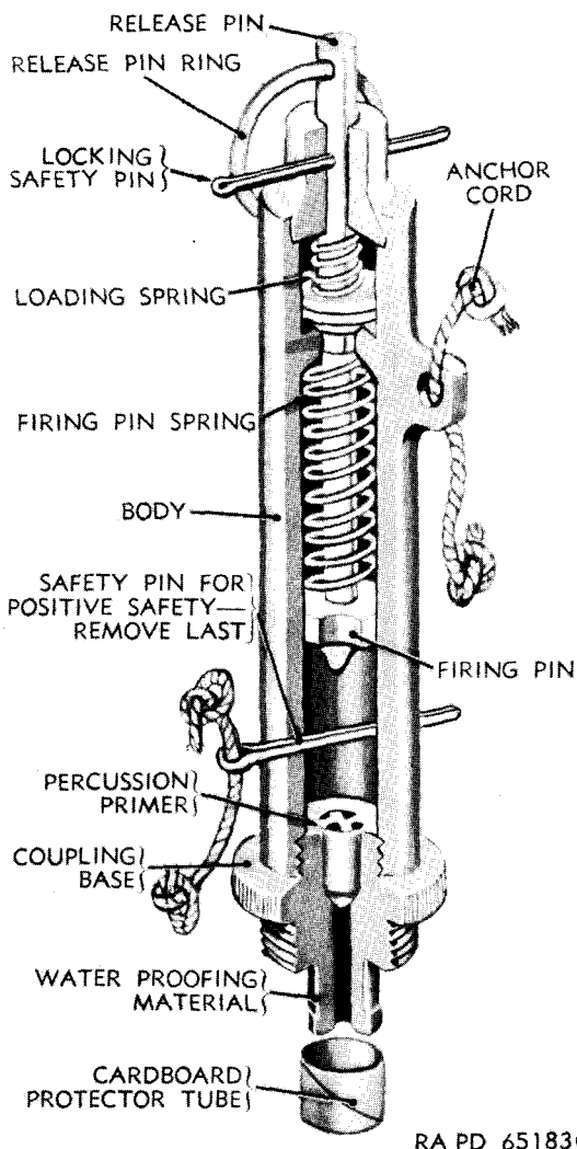
Figure 183. Firing device, pull type, M1.
