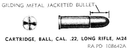
Figure 28. Caliber .22 cartridges.
