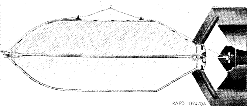
Figure 115. Light case bomb—section.
