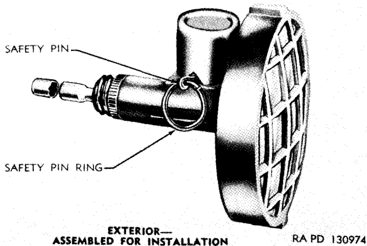
Figure 194. Detonator, concussion type, M1.
