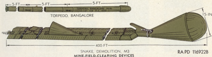
Figure 17. Color identification and typical marking of demolition material.
