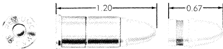
CARTRIDGE, BALL, REVOLVER, CAL. .38, S&W, 146-GRAIN BULLET
