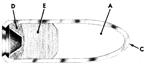
BULLET, TRACER, CARBINE, CAL. .30, M16
