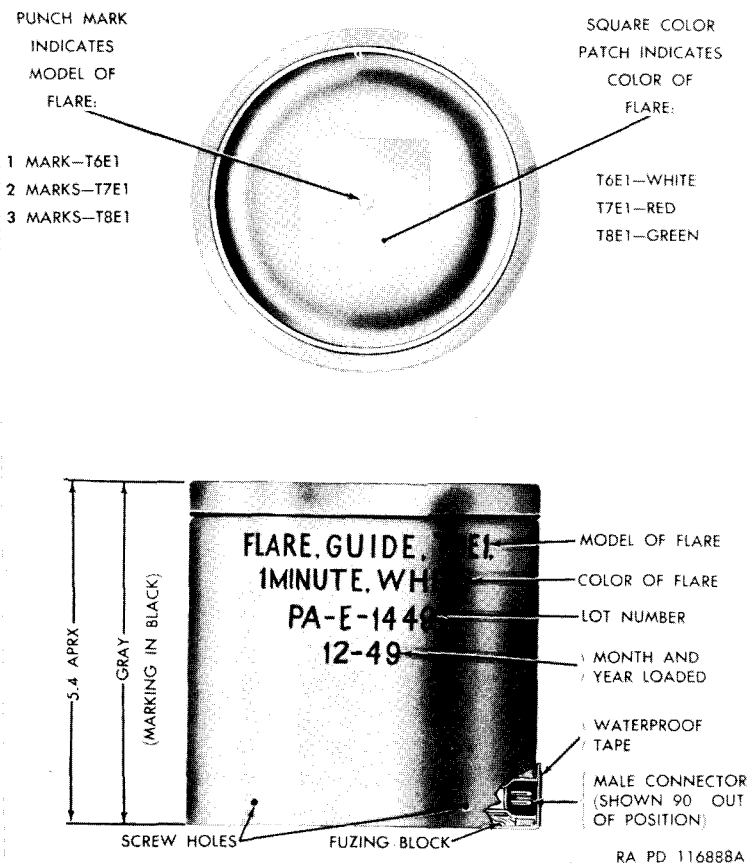
Figure 141. Flare, guide, 1 minute, T6E1 (white).
