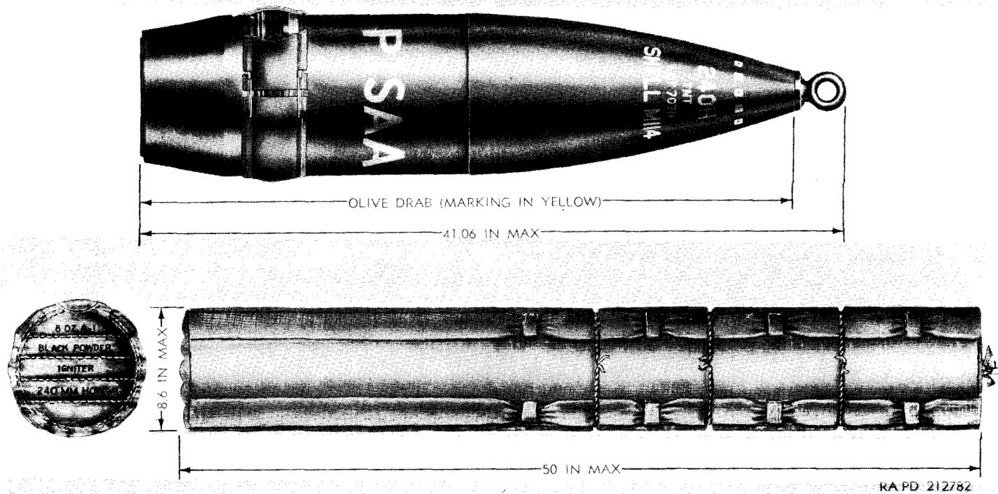
Figure 80. Separate-loading ammunition.
