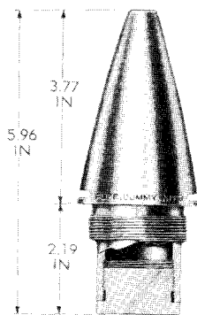
FUZE, DUMMY, M73, FOR 75-MM SUBCALIBER GUN ROUND, 75-MM RIFLE DRILL ROUND, AND 90-MM PRACTICE ROUND
