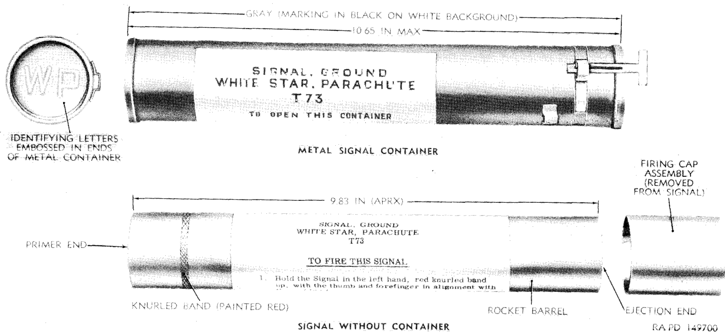
Figure 152. Signal, ground, white star, parachute, M127 (T73).
