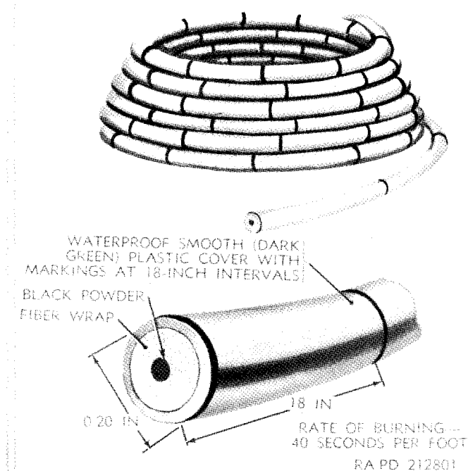
Figure 197. Fuse, safety.
