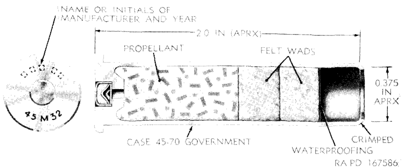
Figure 45. Cartridge, blank, cal .45, M32, line-throwing (Navy).
