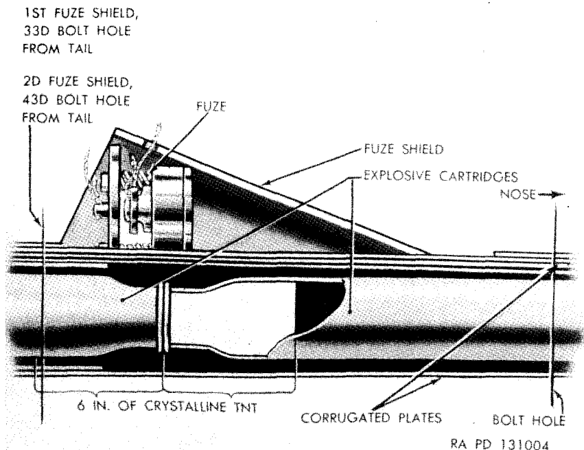
Figure 212. Snake, demolition, M3—longitudinal section at fuze, bullet impact, M1A1.
