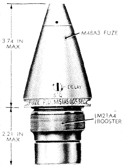
M51A5 PD FUZE 0.05-SEC DELAY IMPACT
