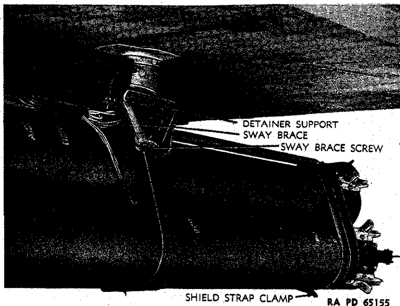
Figure 5—Rear Mount—Front View
